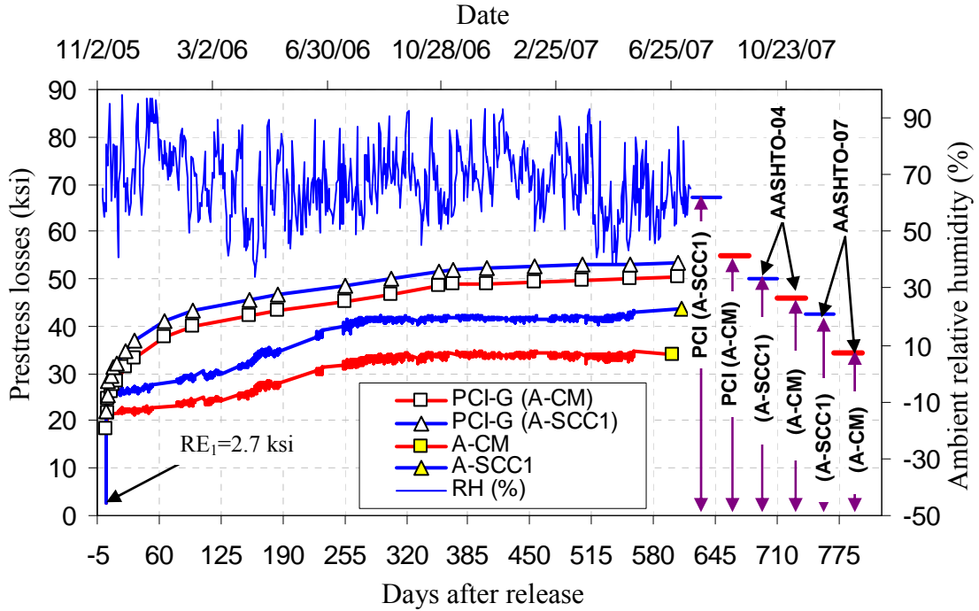
Figure 4-8 Measured and predicted prestress losses for Plant-A girders
