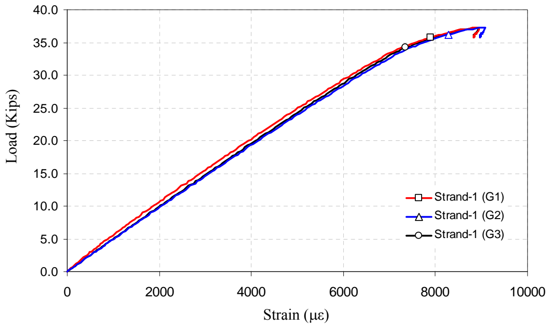
Figure G-3 Load-strain relationship of sample strand-1 Plant-B
