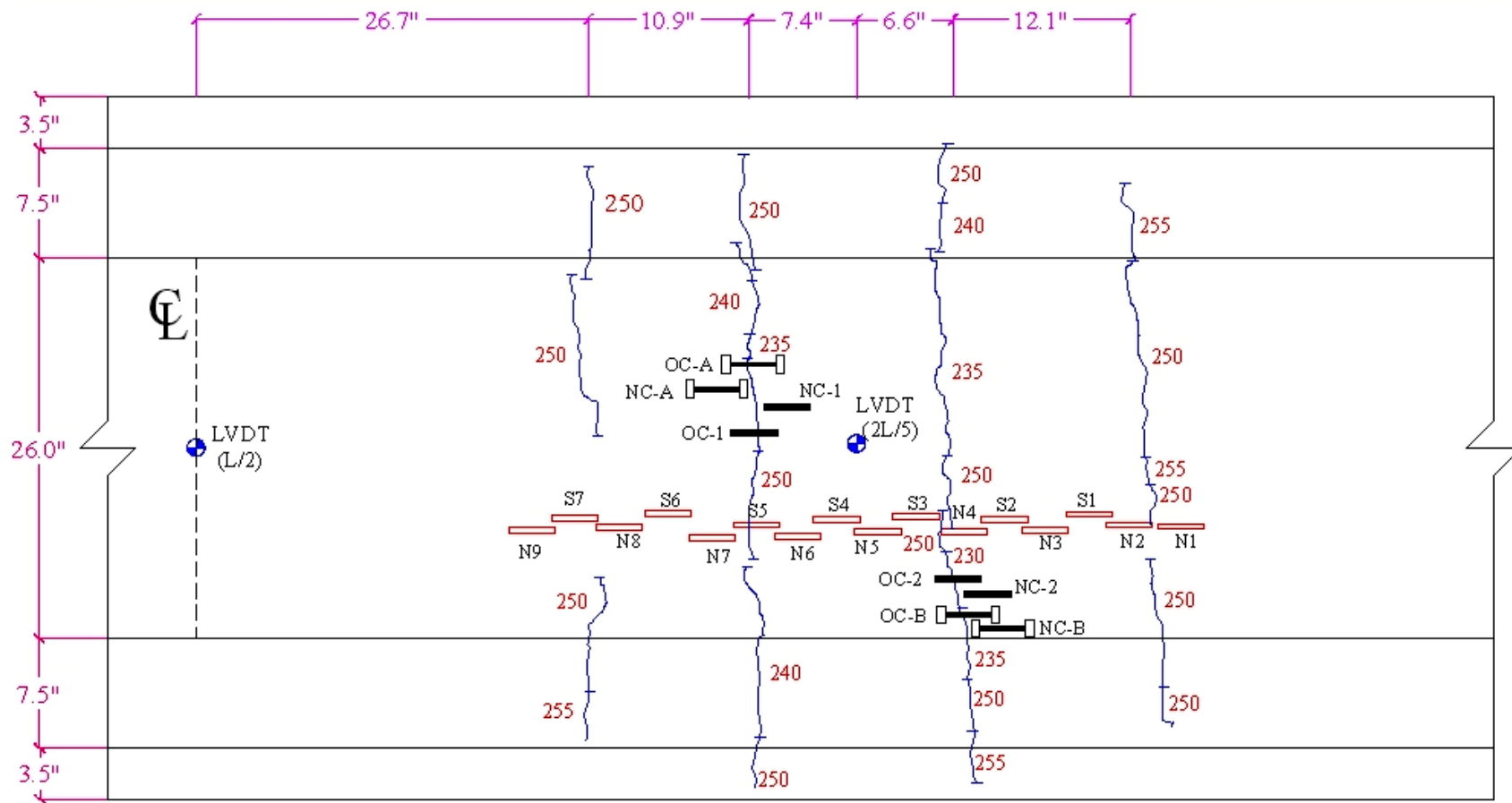
Figure F-4: Location of gages and crack pattern for Girder A-SCC1 (Loading-1)
