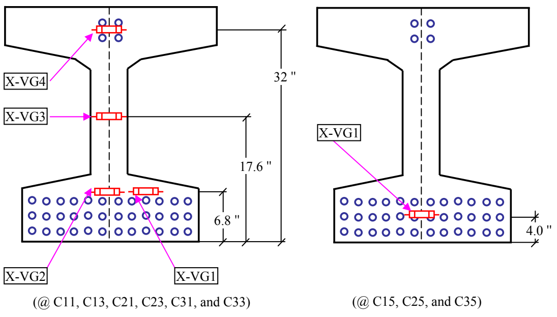
Figure B-8 Plant-B nominal locations of concrete vibrating wire strain gages for measuring longitudinal strains
