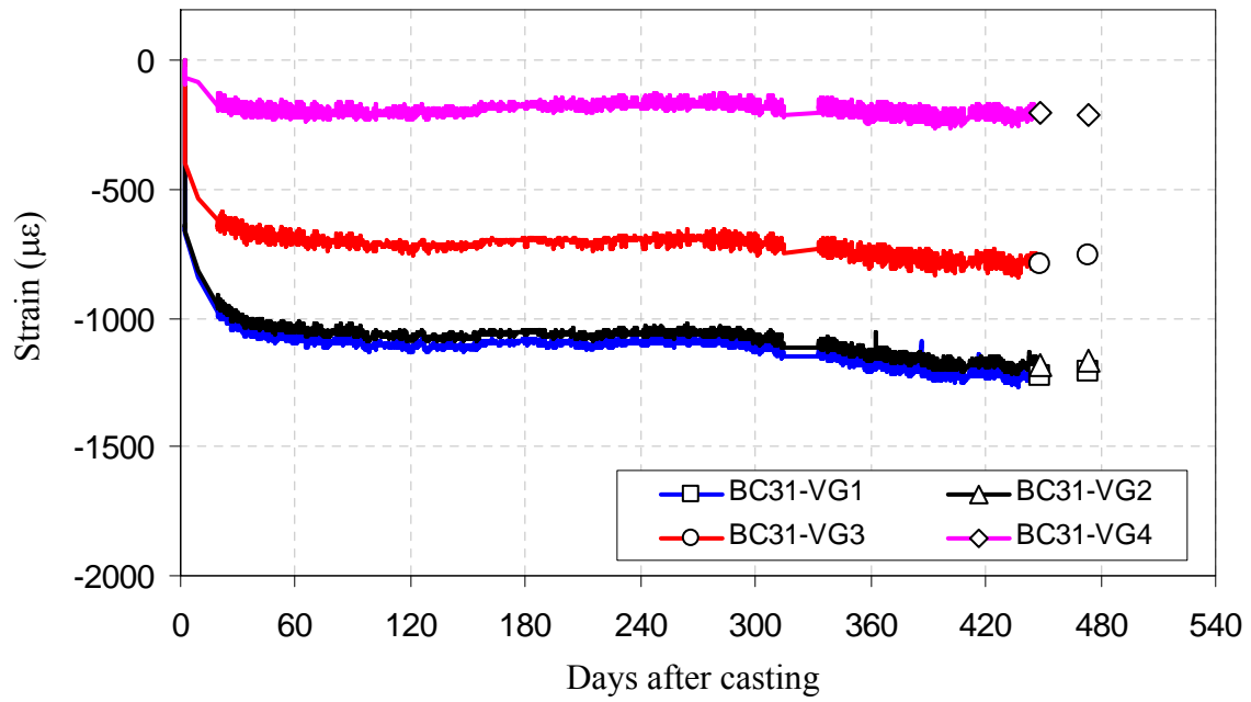
Figure B-32 B-CM strains at L/2
