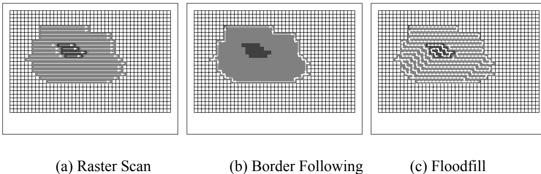
Figure 7. Classic methods for segmentation.
