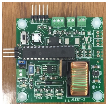
Figure 36: Blinker sign controller circuit.
