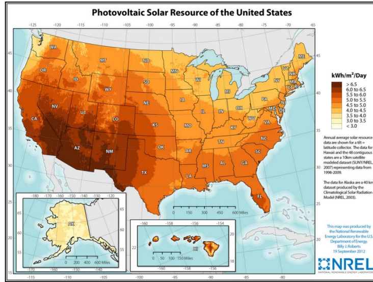
Figure 12: National average PV solar radiation energy map [15].
