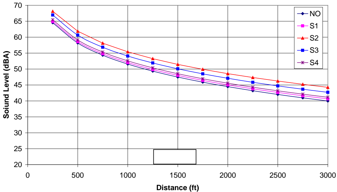
Figure 6.20 Decay of Sound with Distance – Truck
