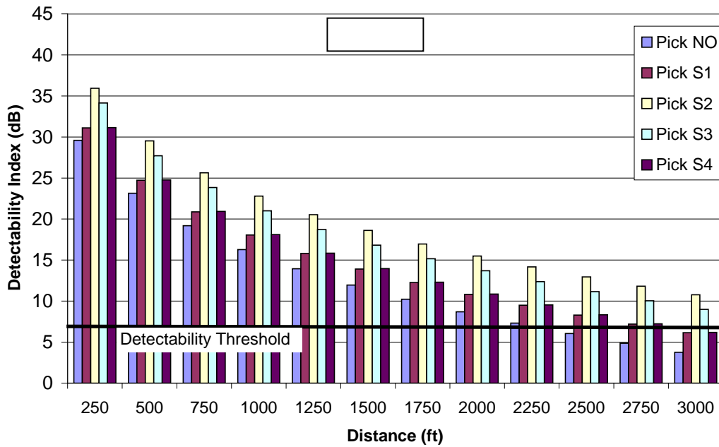
Figure 6.25 Theoretical Detectability of a Pickup
