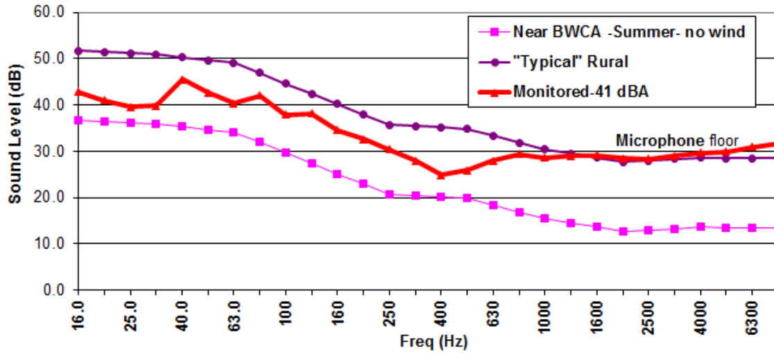
Figure 6.21 Some Typical Quiet Ambient Background Spectra
