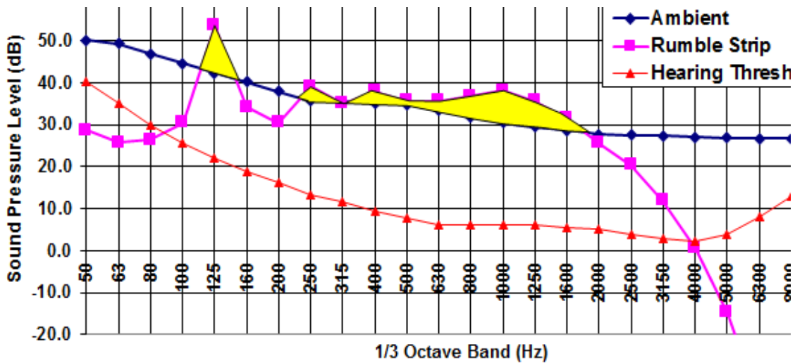
Figure 6.22 Example of Determining Detectability
