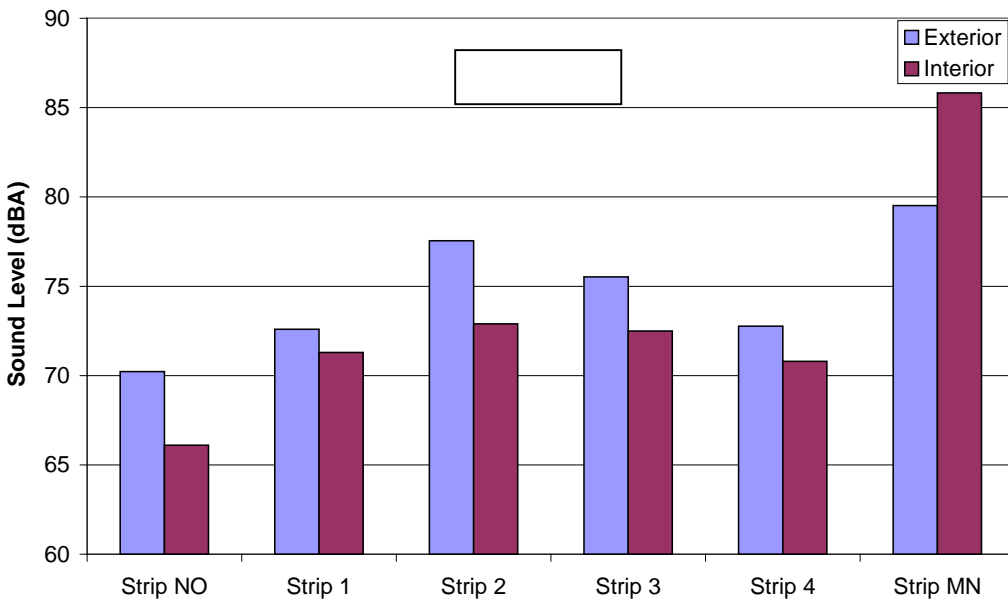
Figure 6.7 Exterior and Interior Sound Levels with the Pickup
