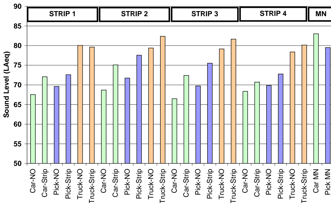
Figure 6.1 Exterior LAeq at 50 feet
