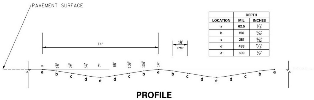
Figure 3.4. Rumble Strip Design 3 (14 inches wide, 1/16 – 1/2 inch depth)
