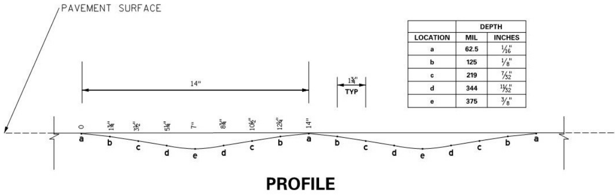
Figure 3.2. Rumble Strip Design 1 (14 inches wide, 1/16 – 3/8 inch depth)
