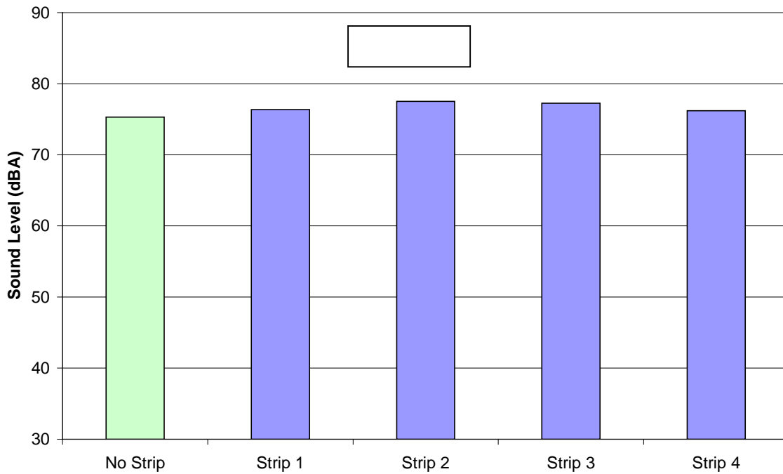
Figure 6.5 Truck – Interior Sound Levels
