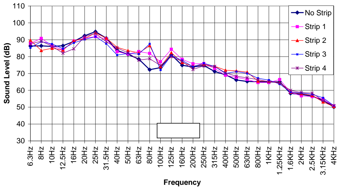
Figure 6.17 Sound Level Spectra a (L10) Inside the Truck
