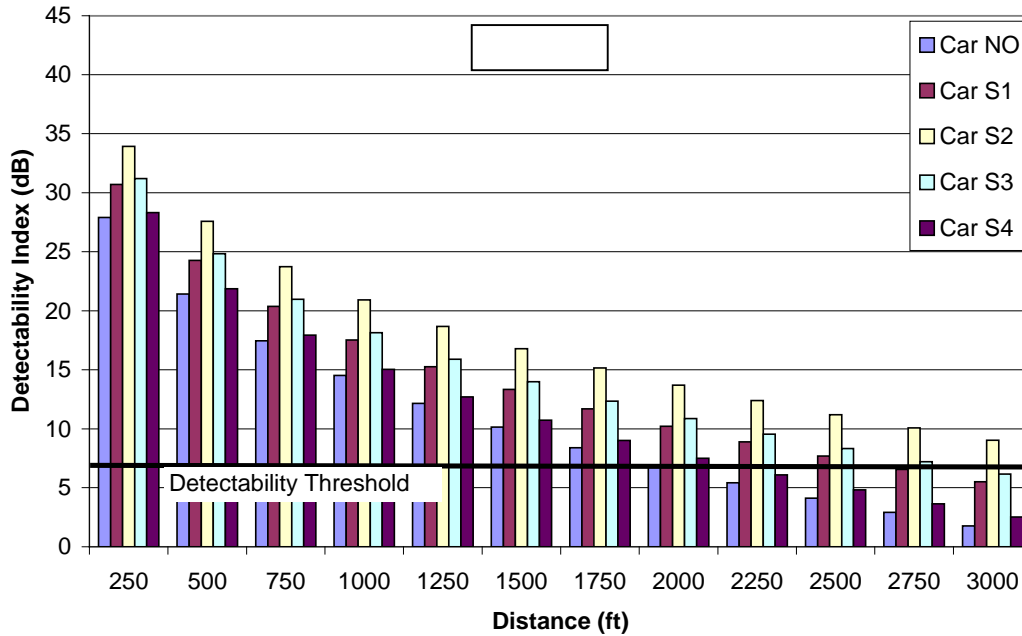
Figure 6.23 Theoretical Detectability of a Passenger Car
