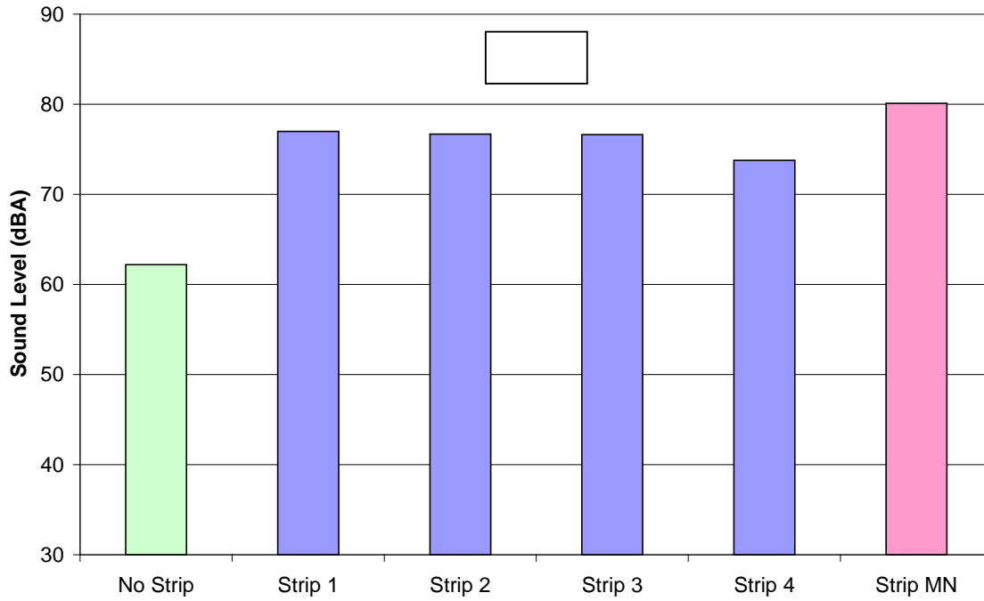
Figure 6.3 Car – Interior Sound Levels
