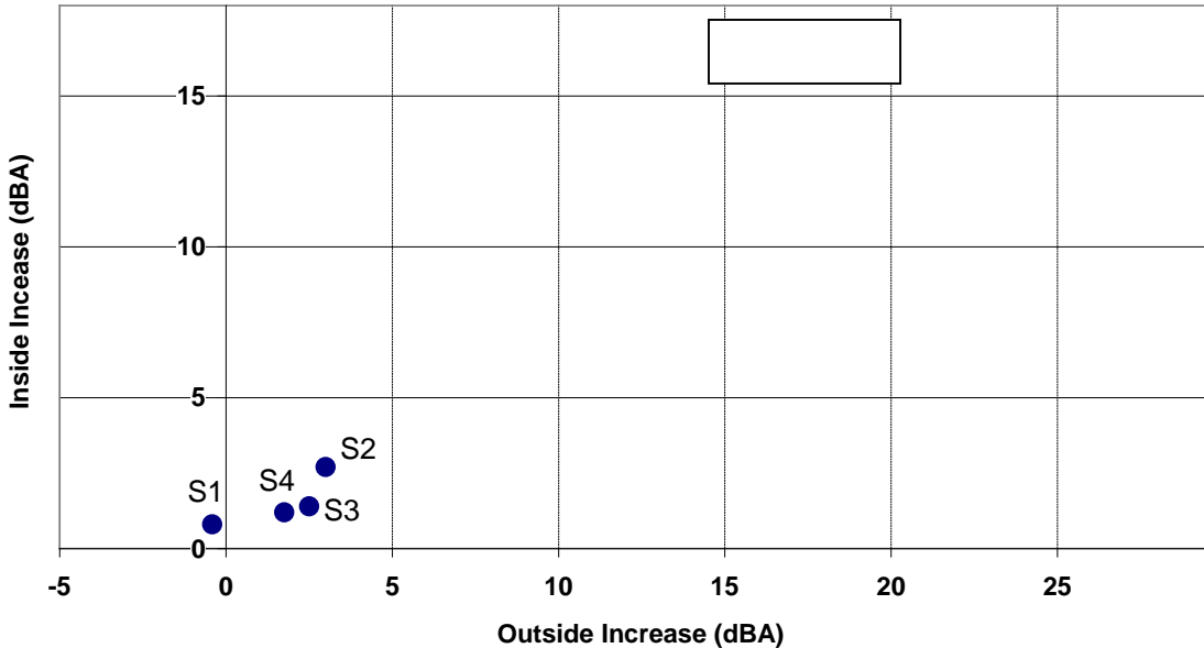
Figure 6.11 Cartesian Plot of Interior vs Exterior Sound Level Increase in the Truck
