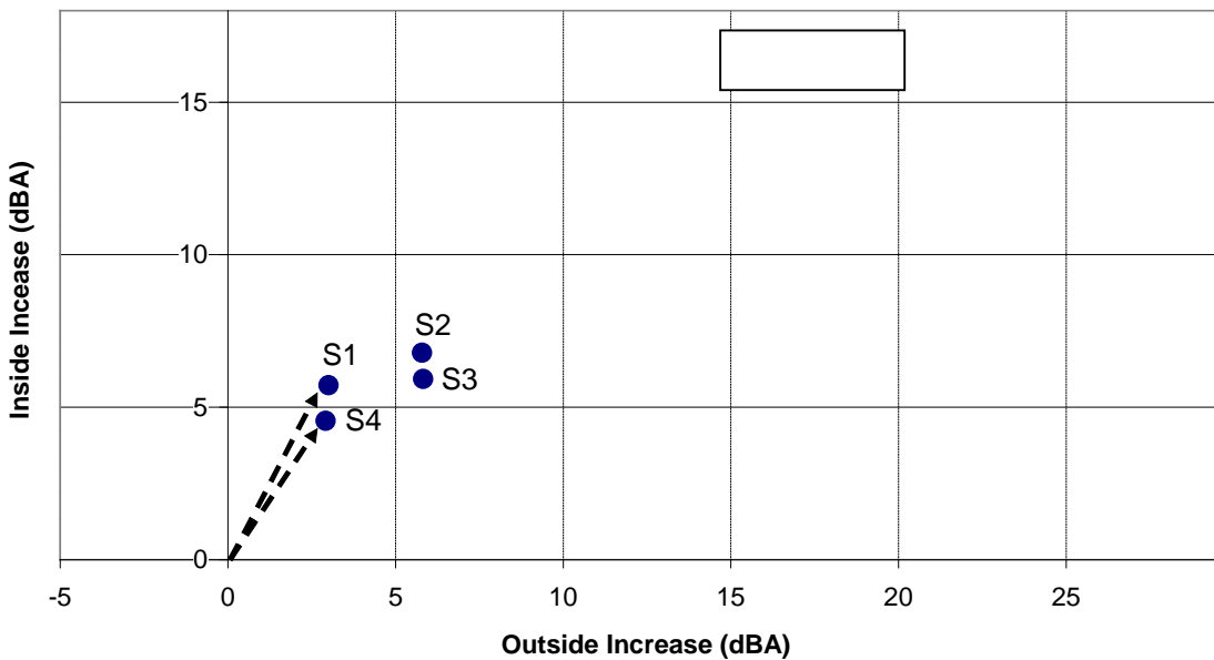
Figure 6.10 Cartesian Plot of Interior vs Exterior Sound Level Increase in the Pickup
