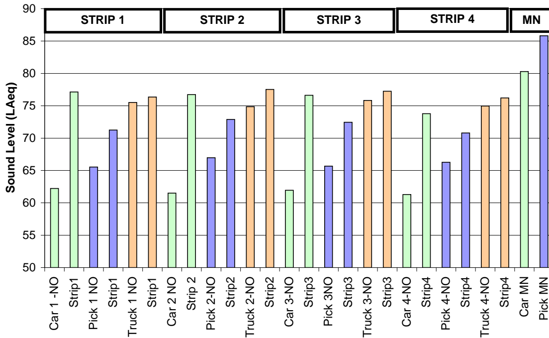
Figure 6.2 Interior LAeq Levels
