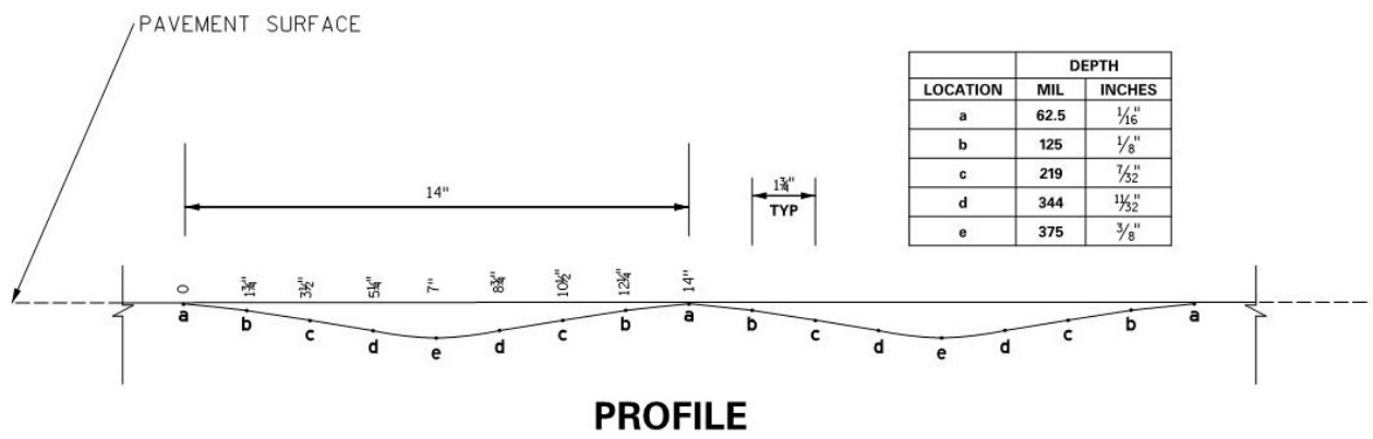
Figure 3.5. Rumble Strip Design 4 (Two 8 inch wide strips 4 inches apart, 1/16 – 3/8 inch depth)
