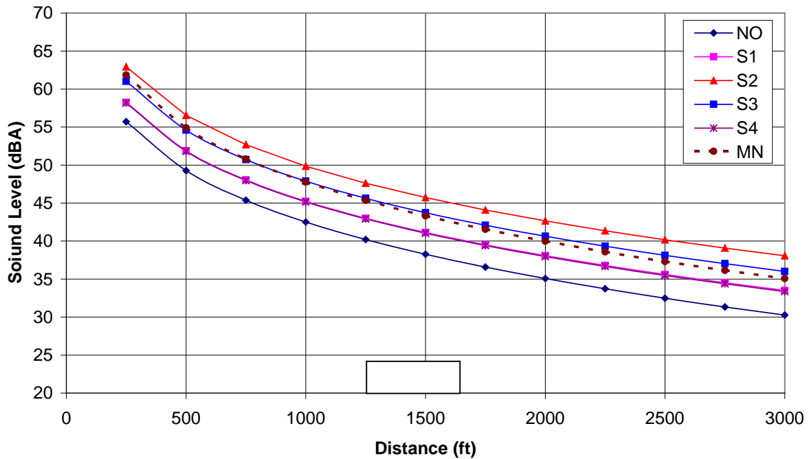
Figure 6.19 Decay of Sound with Distance – Pickup
