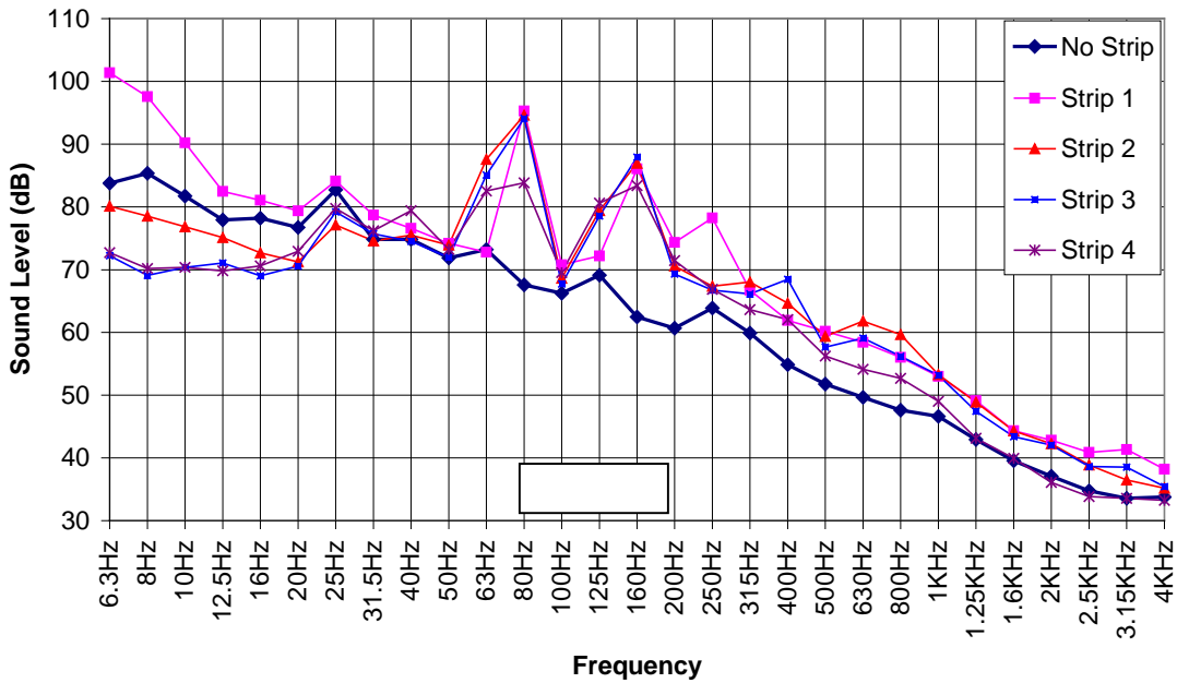
Figure 6.15 Sound Level Spectra a (L10) Inside the Car
