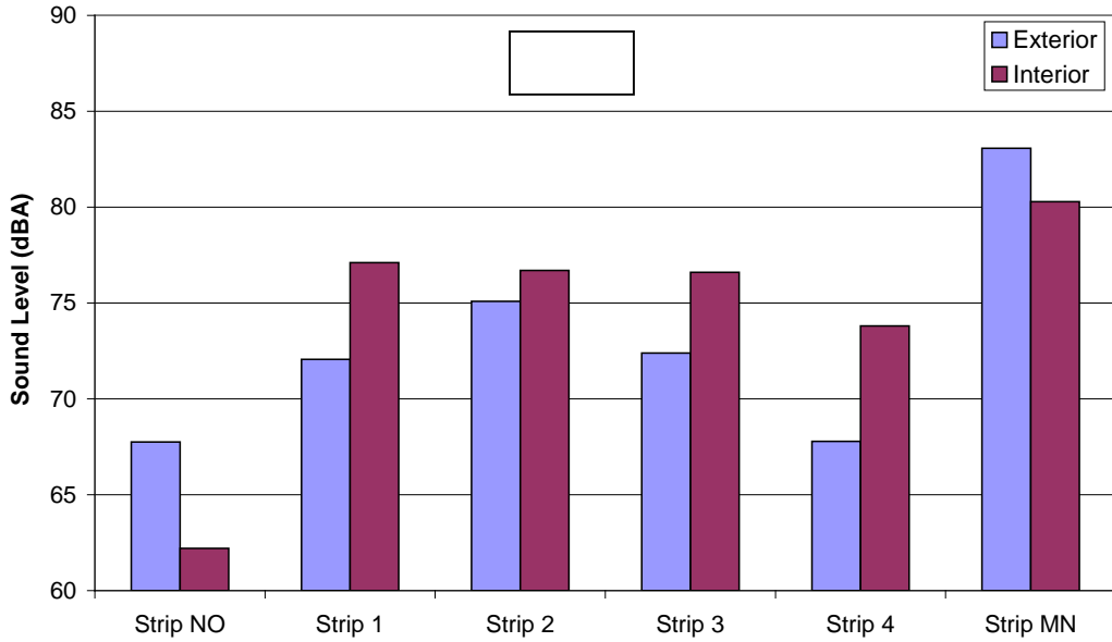
Figure 6.6 Exterior and Interior Sound Levels with the Car
