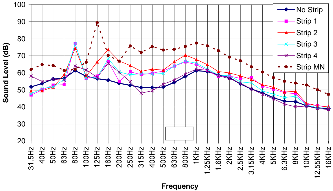
Figure 6.12 Sound Level Spectra a 50 feet of Car Pass-by
