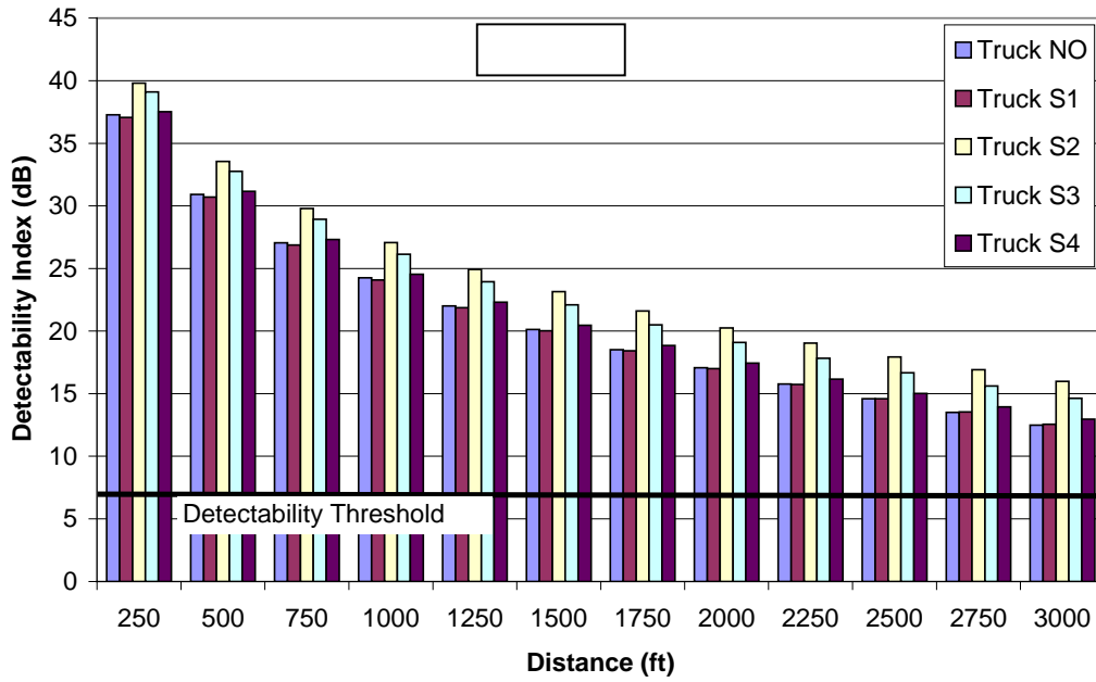
Figure 6.26 Theoretical Detectability of a Truck
