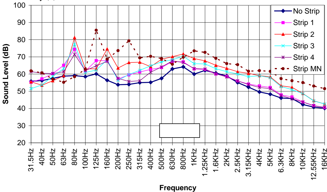
Figure 6.13 Sound Level Spectra a 50 feet of Pickup Pass-by
