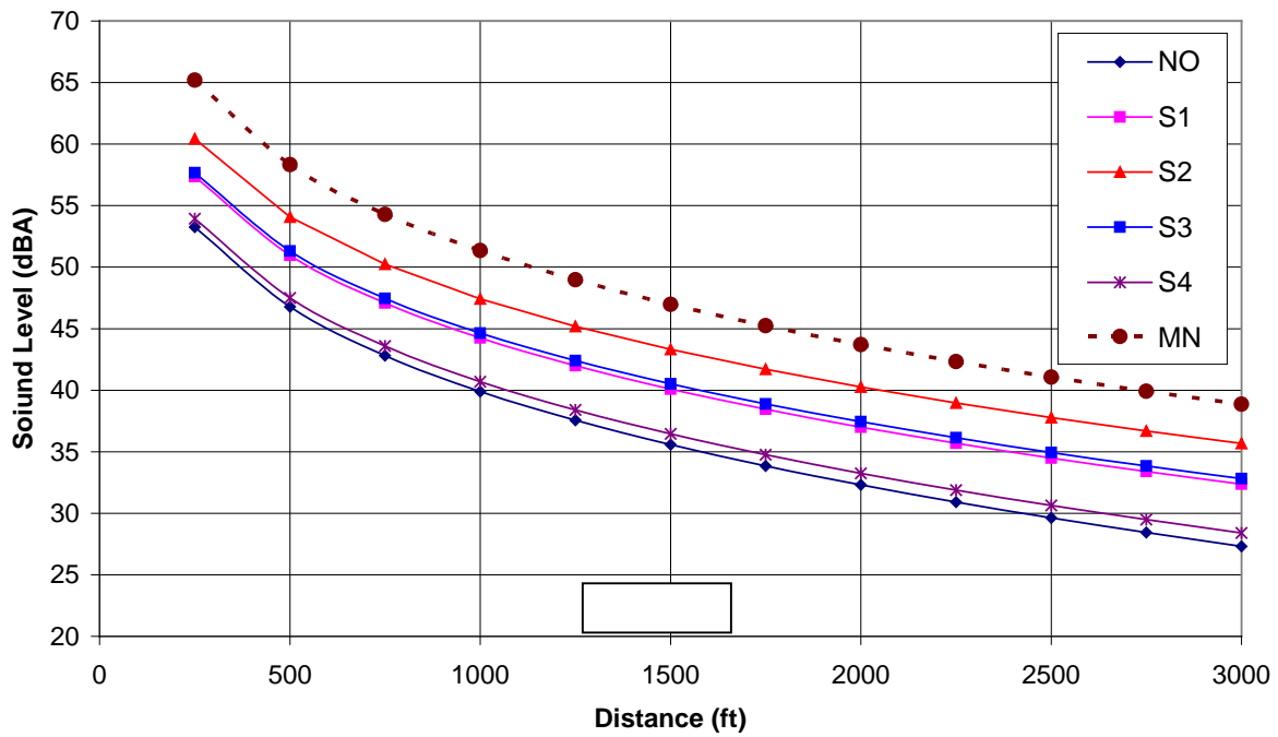
Figure 6.18 Decay of Sound with Distance – Car
