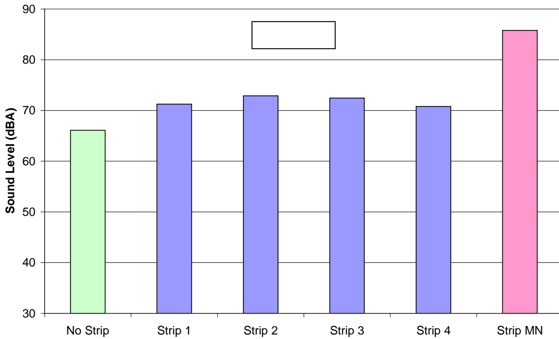
Figure 6.4 Pickup – Interior Sound Levels
