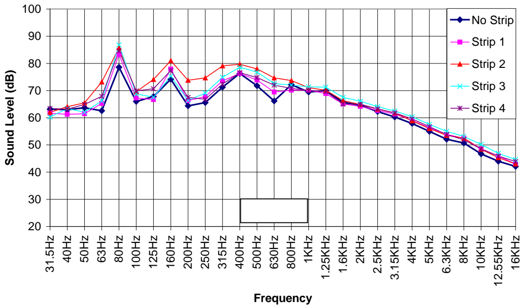
Figure 6.14 Sound Level Spectra at 50 ft of Truck Pass-by
