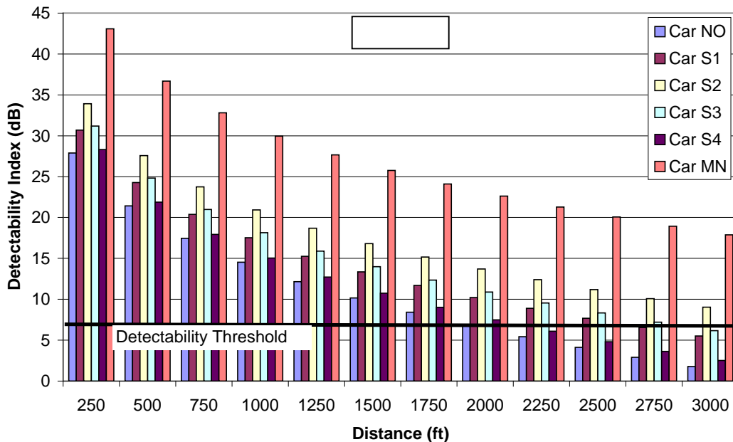
Figure 6.24 Theoretical Detectability of a Passenger Car with a Minnesota Strip
