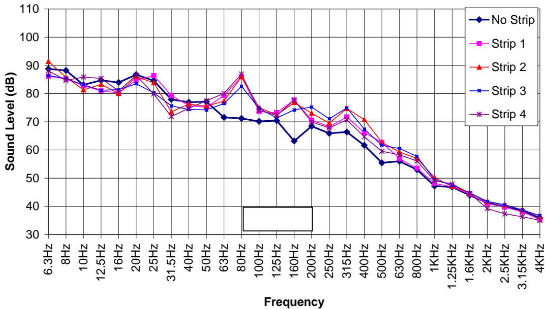
Figure 6.16 Sound Level Spectra a (L10) Inside the Pickup
