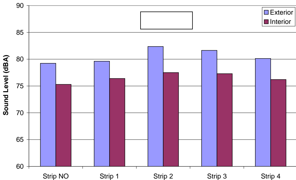
Figure 6.8 Exterior and Interior Sound Levels with the Truck
