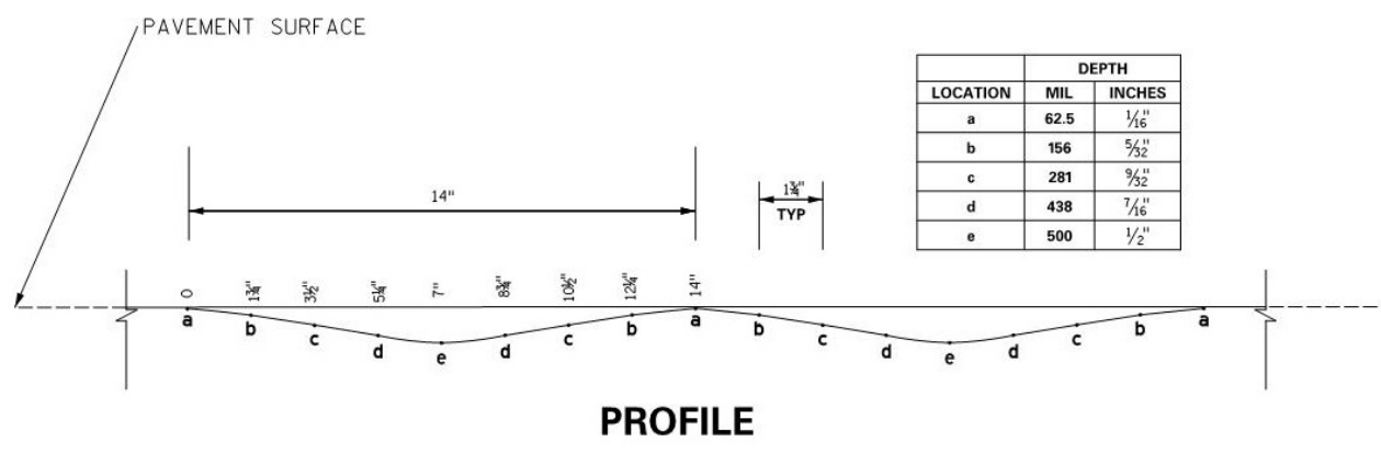
Figure 3.3. Rumble Strip Design 2 (Two 8 inch wide strips 4 inches apart, 1/16 – 1/2 inch depth)
