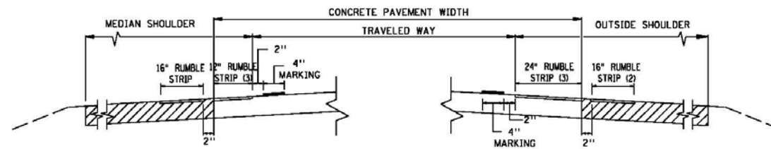
FIGURE 3C CONCRETE FREEWAY/MULTI-LANE OPTION A (ONE ROADWAY SHOWN)
