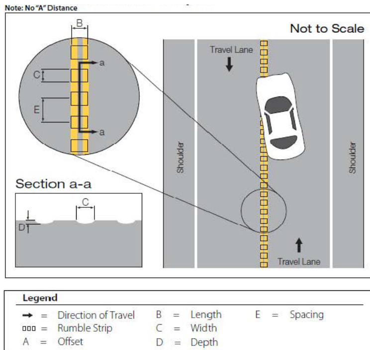
Figure 4. Centerline Rumble Strips
