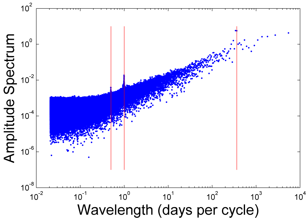
Figure 6.4: Single-sided amplitude spectrum of temperatures from Cell #10, Sensor 11. This is a PCC cell on the Mainline, and the sensor is 2.4293 m (7.97 ft) below the surface in the clay subgrade. The vertical red lines show wavelengths of \frac{1}{2} day, 1 day and 1 year.
