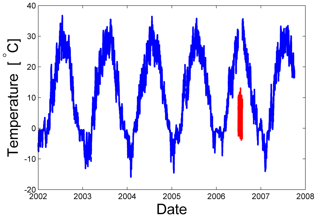
Figure 6.5: Temperature data from Cell #6, Sensor 5 during 2002 through 2007. The red markers show the data that is flagged by the “out of range” test. This test correctly identifies the anomalous data in the summer of 2006, even though all of the data is within the range of normal annual variation.
