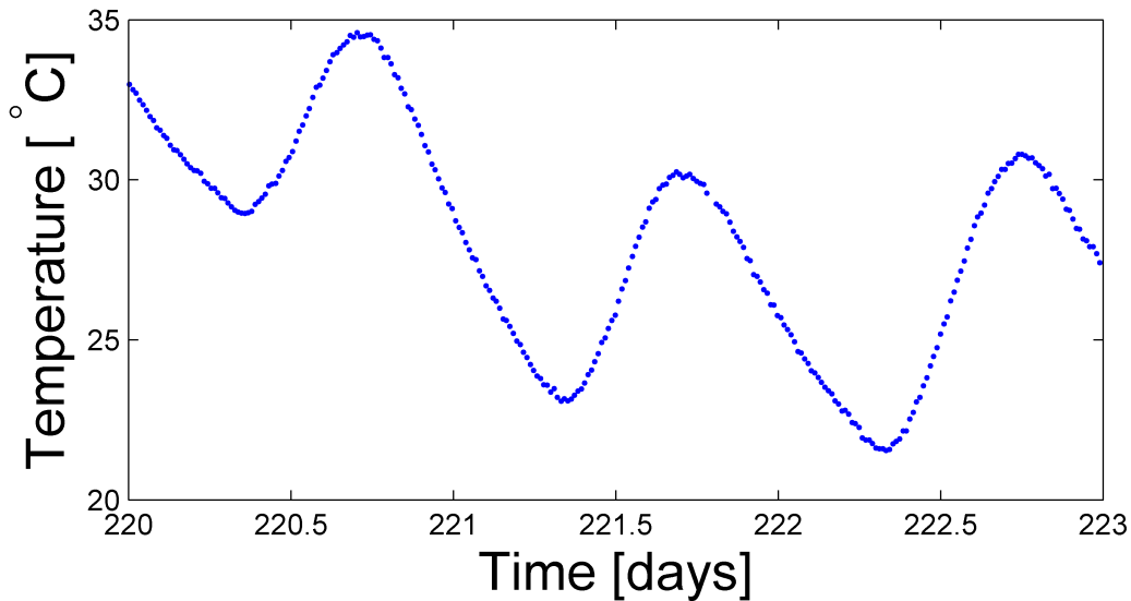
Figure 2.5: The anticipated diurnal variation is emphasized in this temperature data plot for a few days from Cell #10, Sensor 3. Shown are 285 raw measurements taken in the summer of 2001, with a 15 minute collection interval.
