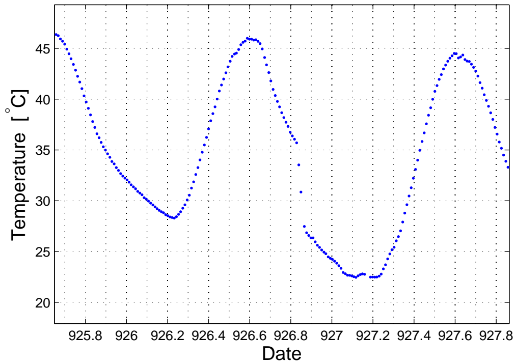
Figure 3.9: Cell #40, Sensor 1 is shown. The data shows an unrealistic, abrupt, change in temperature – dramatically deviating from the underlying sinusoidal trend. Often, this appears as though the sensor is suddenly calibrated differently. A possible explanation for such behavior, in shallow sensors during summer months, is a passing late-afternoon rainstorm.
