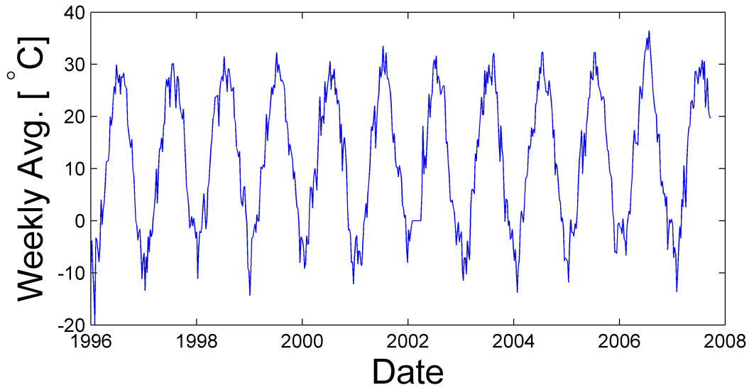
Figure 2.6: The anticipated annual variation is emphasized in this temperature data plot for 592 weekly averages of raw measured temperatures from Cell #10, Sensor 3. The anticipated annual (seasonal) variation dominates the underlying trend, although weather variations can be seen.
