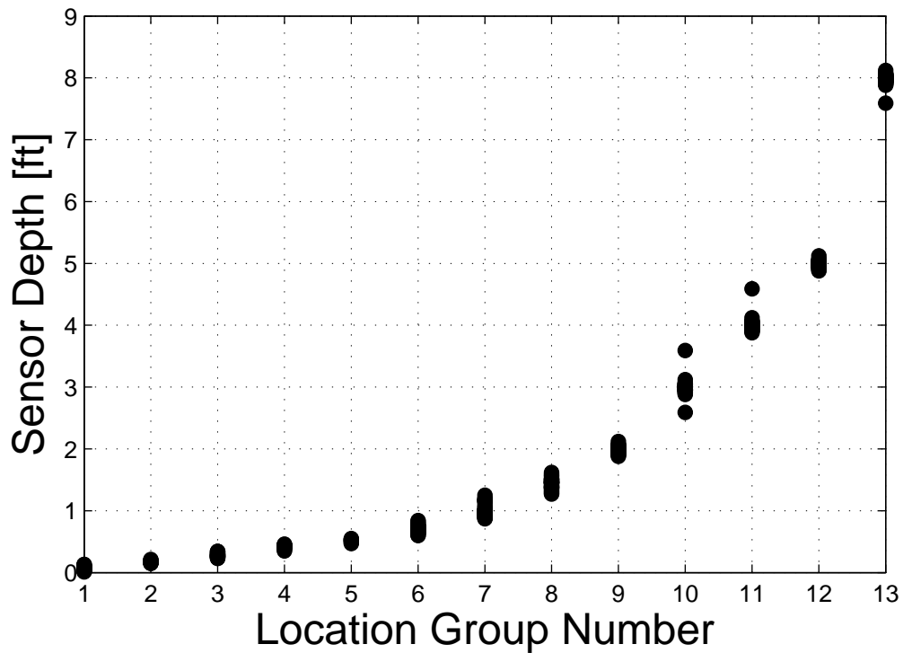
Figure 4.1: A black disk is plotted for each sensor in the HMA cells. This shows the range of sensor depths for each of the 13 Mn/DOT -defined Location Groups. There is some overlap between the groups.
