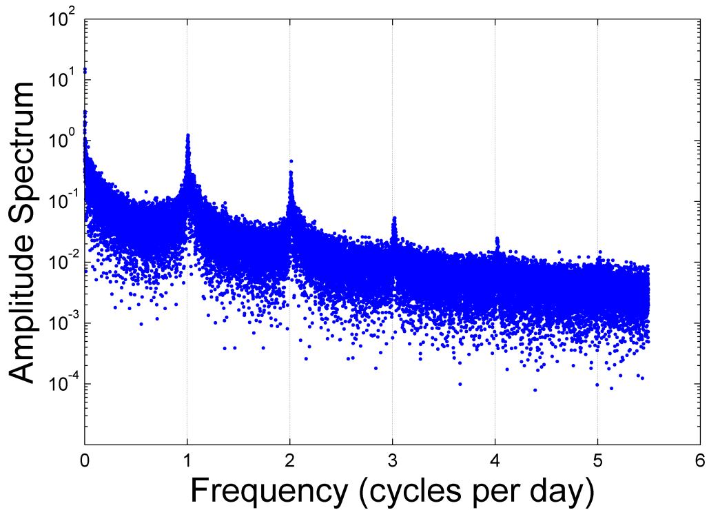
Figure 6.1: Single-sided amplitude spectrum of temperatures for the complete data record (1996-2007) from Cell #1, Sensor 1. This is an HMA cell on the Mainline, and the sensor is 0.0305 m (0.1 ft) below the surface.
