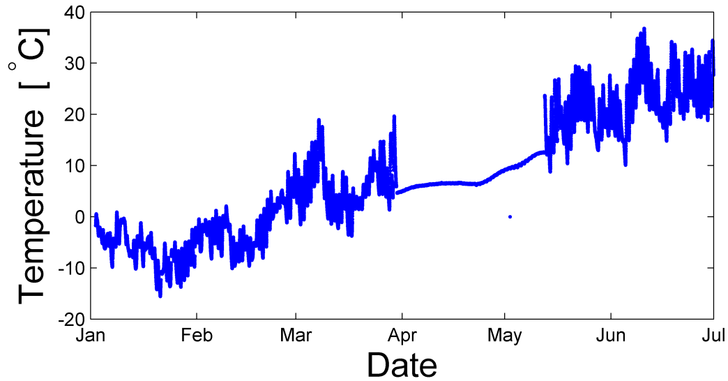
Figure 6.12: This shows the first half of 2001 for Cell #15, Sensor 3. The months of April and May present an example of hypovariate data. The overall trend through these months is correct, and the individual temperature values are reasonable (with the exception of the one aberrant point) when viewed in isolation, but the expected diurnal variation has disappeared.
