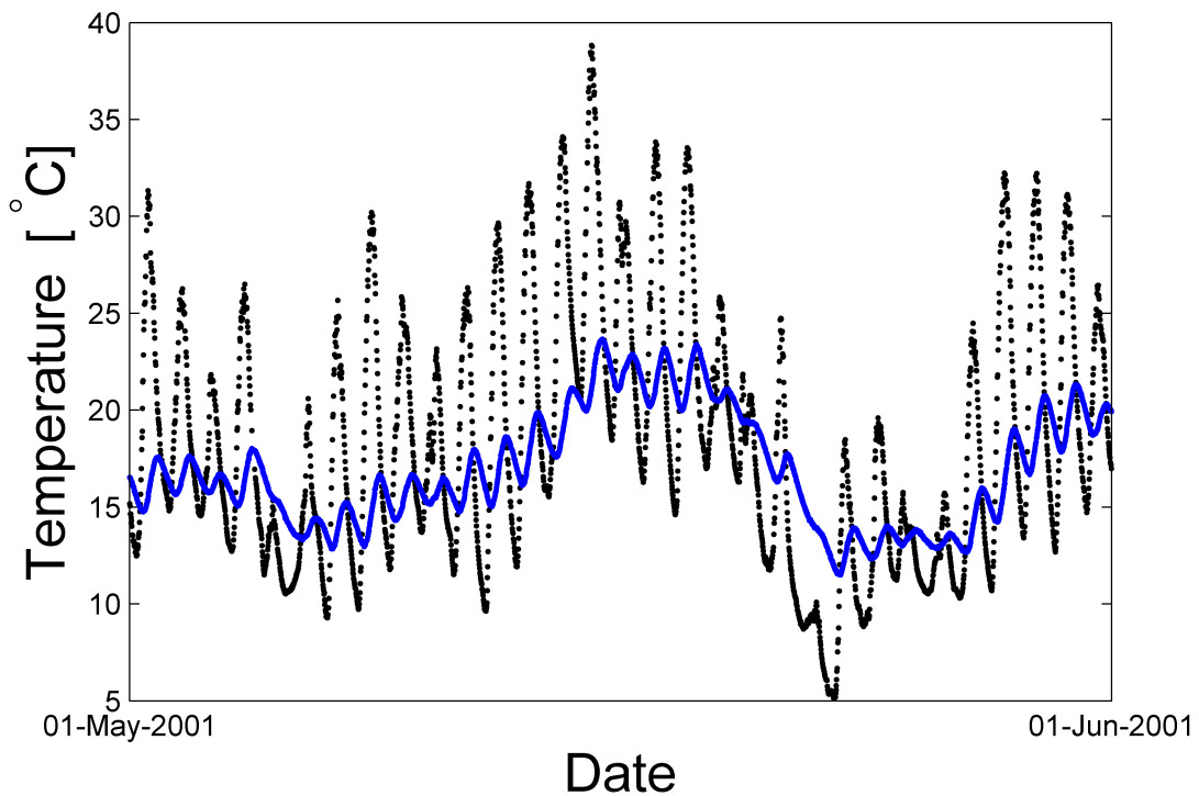
Figure 6.10: Data from May 2001. The blue line shows the recorded temperature record for Cell #4, Sensor 31. The black line shows the median temperature record for all sensors in the same subset (i.e. sensors at the same depth, on the Mainline roadway, in hot mix asphalt cells). The data from Cell #4, Sensor 31 are dramatically less variable (hypovariate) than would be expected; as such, they are flagged by the point extremes test.
