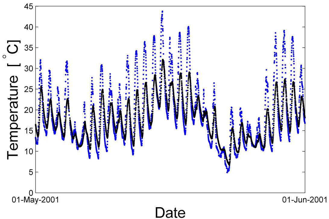
Figure 6.11: Data from May 2001. The blue line shows the recorded temperature record for Cell #4, Sensor 32. The black line shows the median temperature record for all sensors in the same subset (i.e. sensors at the same depth, on the Mainline roadway, in hot mix asphalt cells). The data from Cell #4, Sensor 32 are dramatically more variable (hypervariate) than would be expected; as such, they are flagged by the point extremes test.
