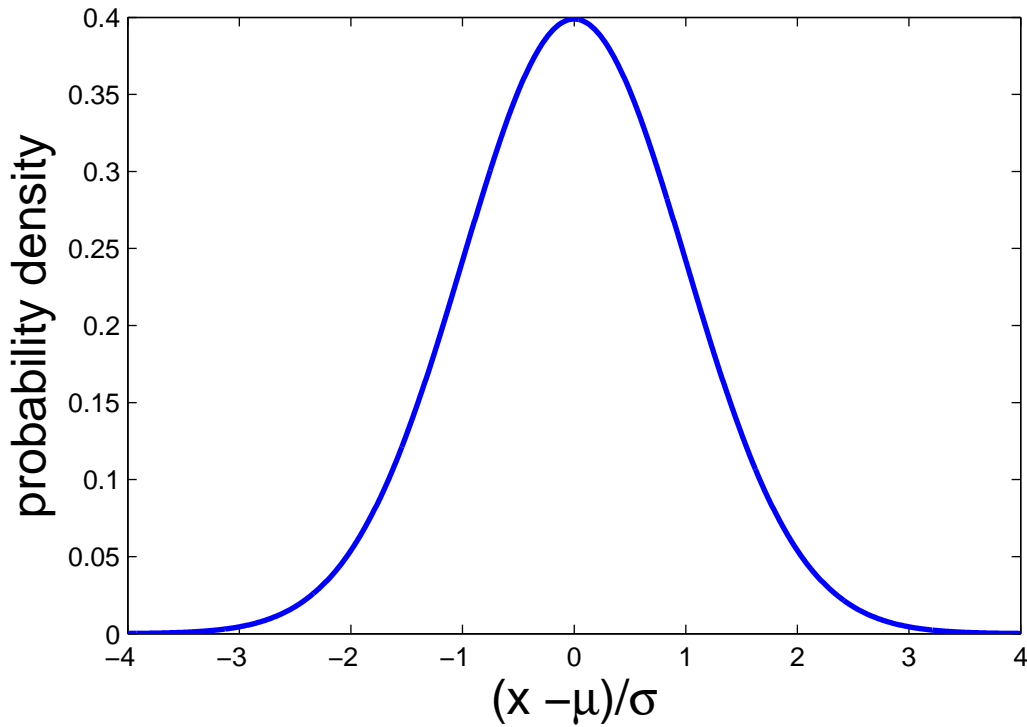
Figure 5.1: Normal distribution probability density function.
