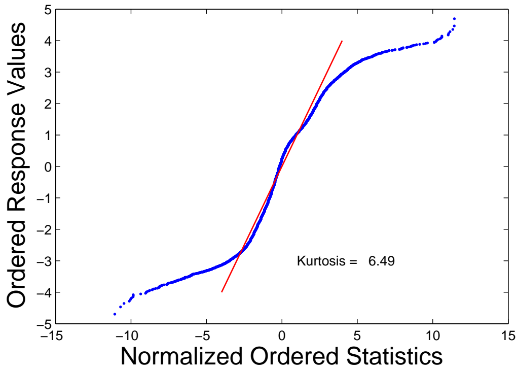
Figure 7.2: A representative Normal probability plot of lag-one data for Cell #5, Sensor 1. The red line represents a theoretical Normal distribution, the blue dots are the measured data.
