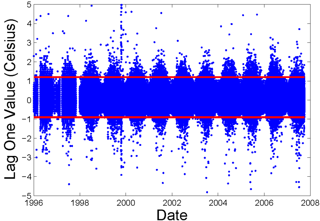
Figure 7.4: A representative plot the Lag-one-versus-time data from Cell #5, Sensor 1. The blue dots show the measured data; the red lines depict the 1st and 99th percentiles of the data.
