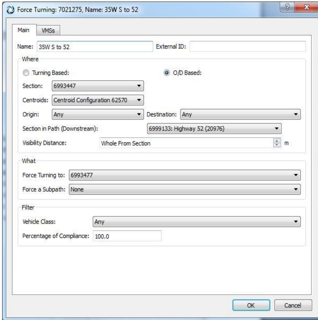
Figure 20. Forced turning dialog menu in Aimsun.
