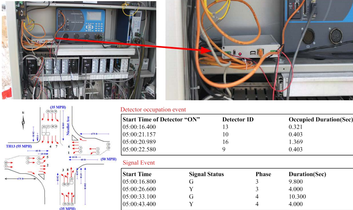
Figure 2.2 Illustration of field installation of Type 2 DCU and data sample
