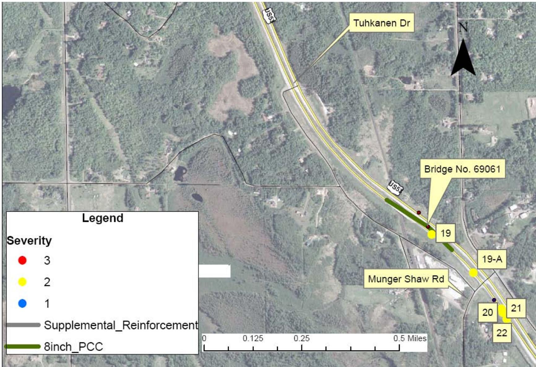
Figure 5.6. TH 53 Distress Map [Munger Shaw Rd to Tuhkanen Dr.], April 2009 (Farm Service Agency, 2002)
