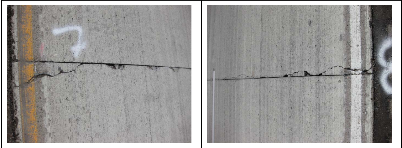
Figure A.4. Distress No. 7 [Left] & No. 8 [Right], April 2009
