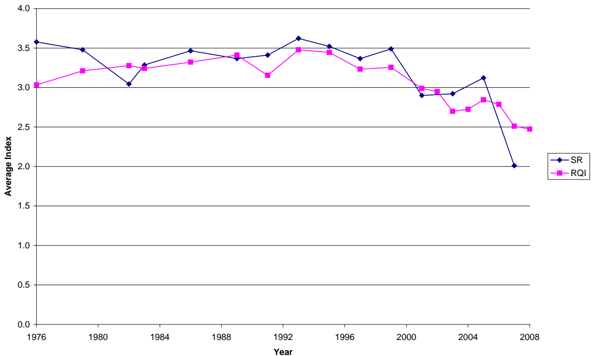
Figure 3.5. Average Pavement Condition Prior to Overlay
