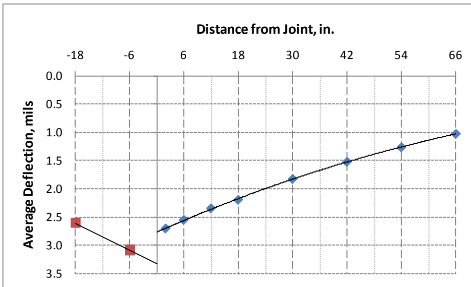
Figure 4.4. Average Deflection Basin when the Load Plate is Before the Joint
