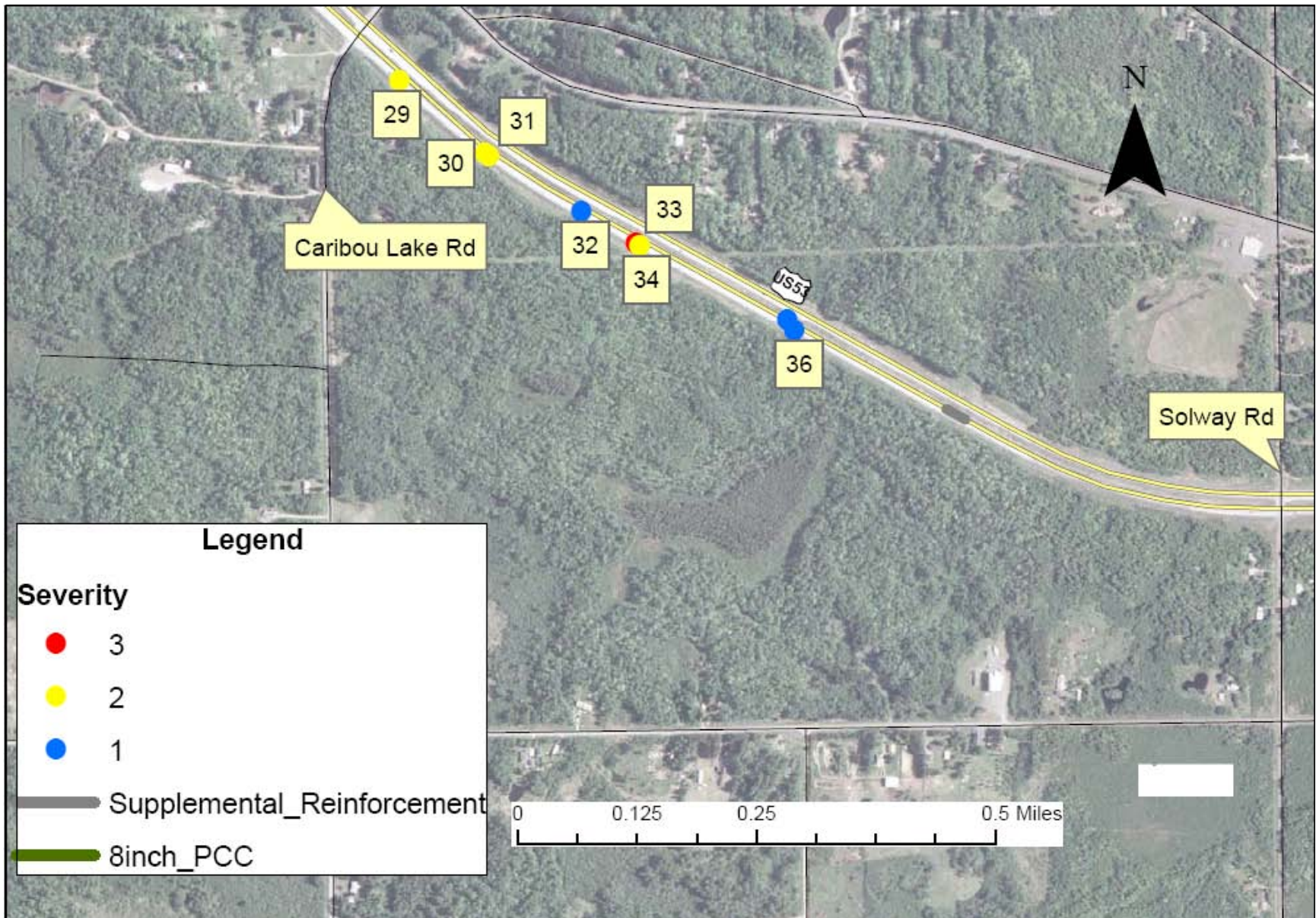
Figure 5.4. TH 53 Distress Map [Solway Rd to Caribou Lake Rd], April 2009 (Farm Service Agency, 2002)
