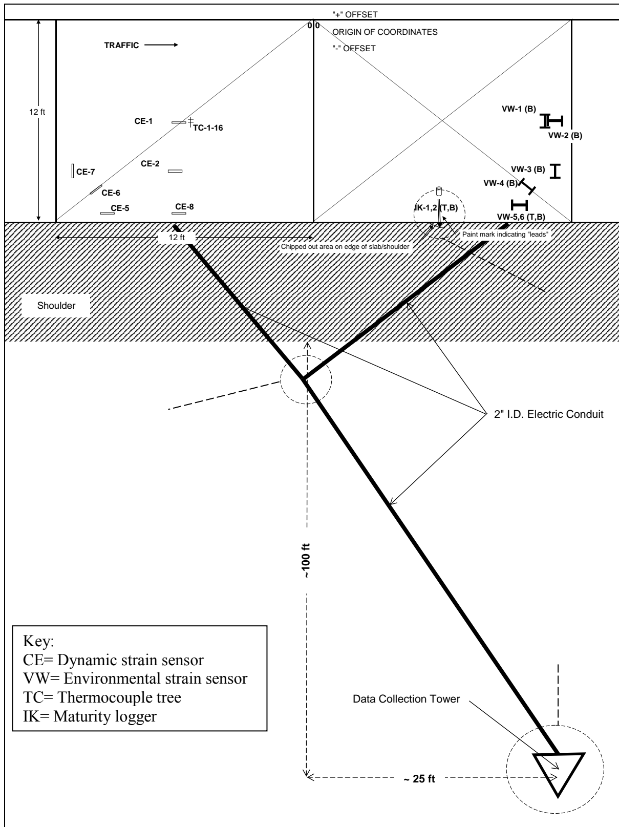
Figure 2.2. Cell 53-1 Instrumentation and Data Collection System Layout
