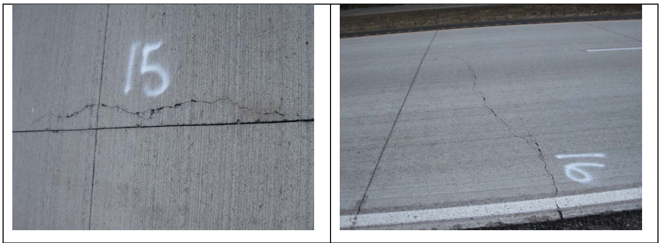
Figure A.8. Distress No. 15 [Left] & No. 16 [Right], April 2009
