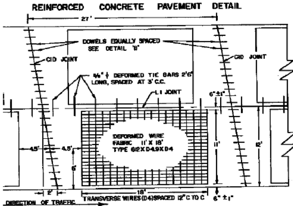
Figure 3.3. Reinforced Concrete Pavement Detail for 1972 TH 53 Project
