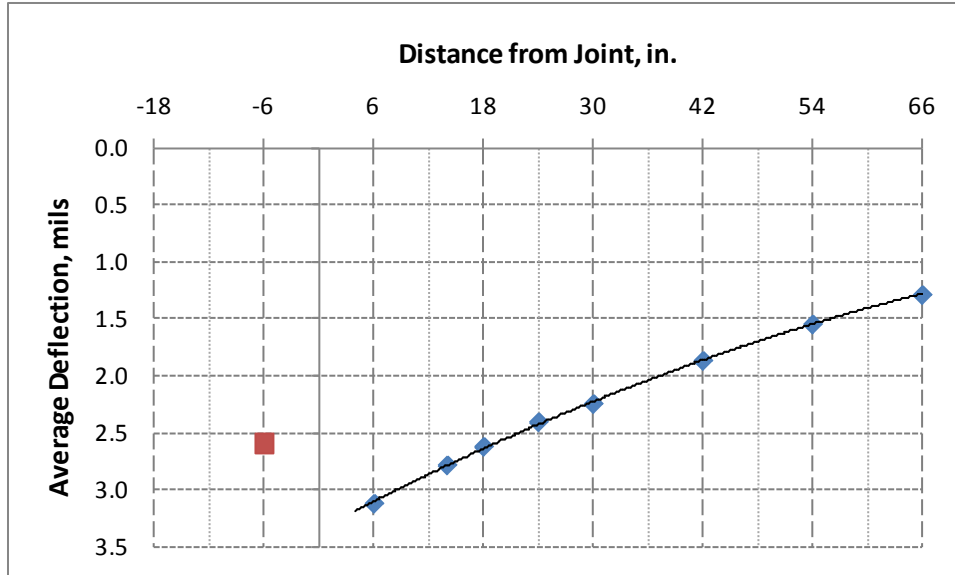
Figure 4.5. Average Deflection Basin when the Load Plate is After the Joint
