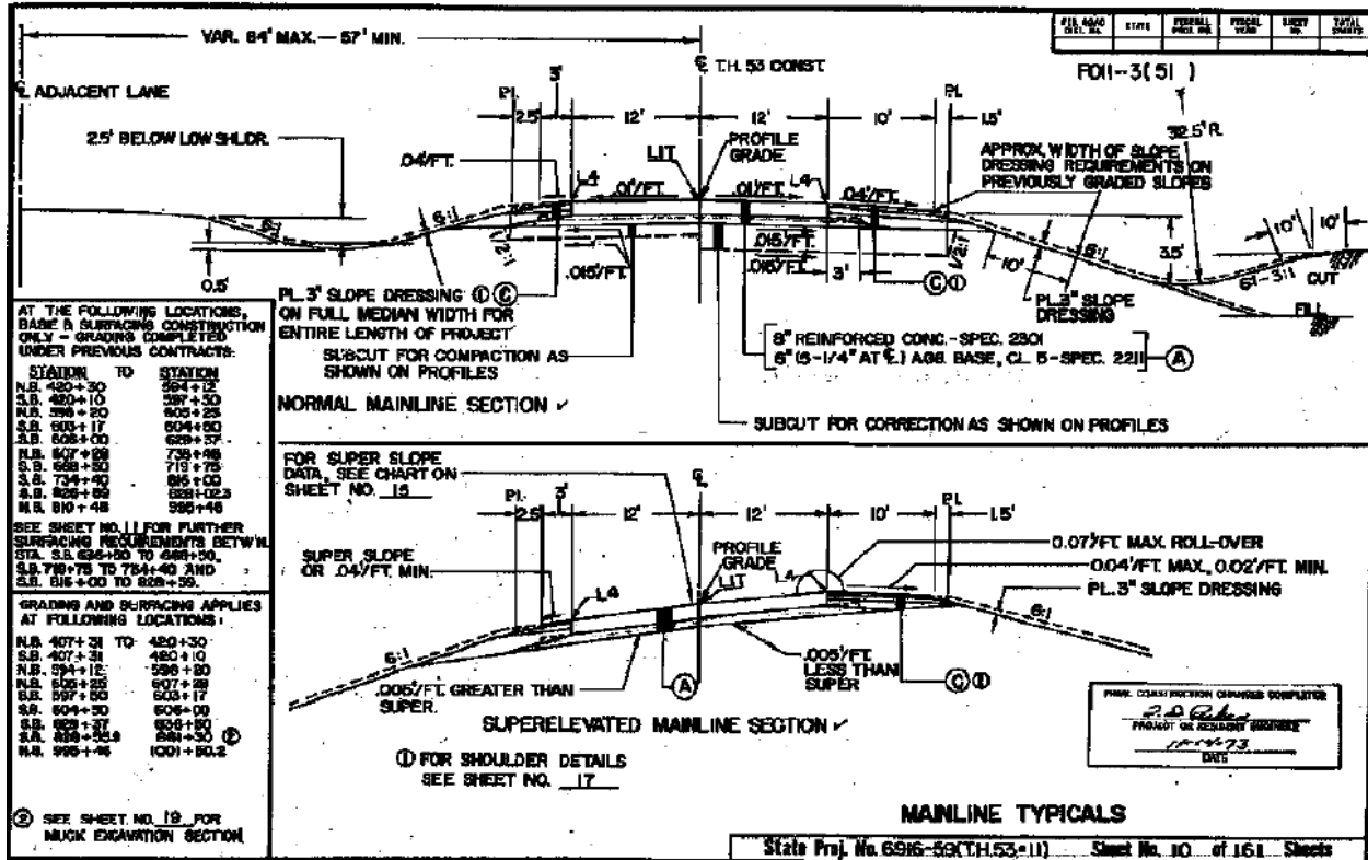
Figure 3.2. Mainline Typical Sections for 1972 TH 53 Project
