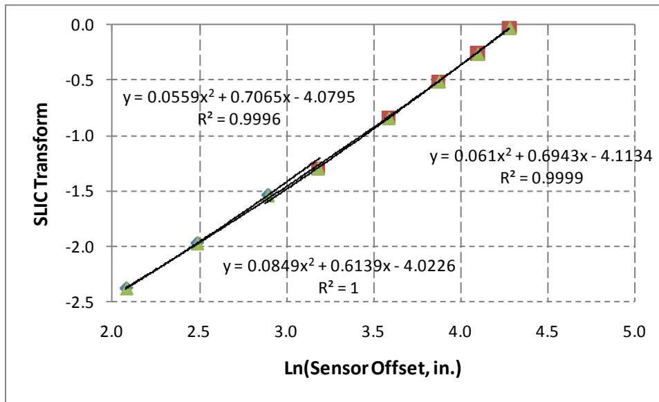
Figure 4.2. SLIC Check of Mid-Panel Deflection Data
