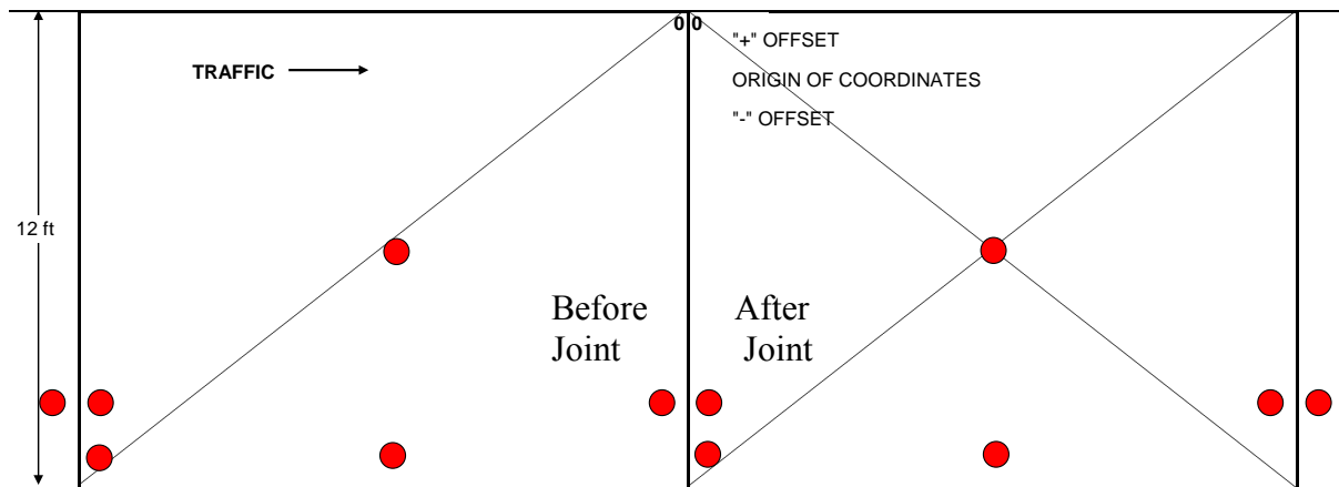
Figure 4.1. Routine FWD Testing Locations in Test Cell 53-1
