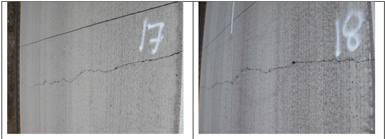
Figure A.9. Distress No. 17 [Left] & No. 18 [Right], April 2009
