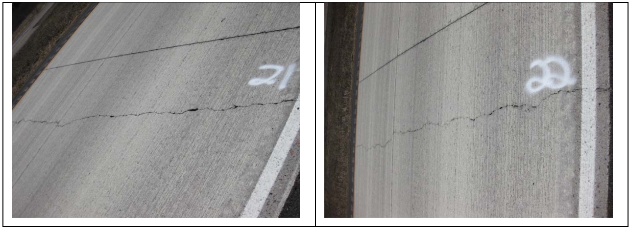
Figure A.11. Distress No. 21 [Left] & 22 [Right], April 2009
