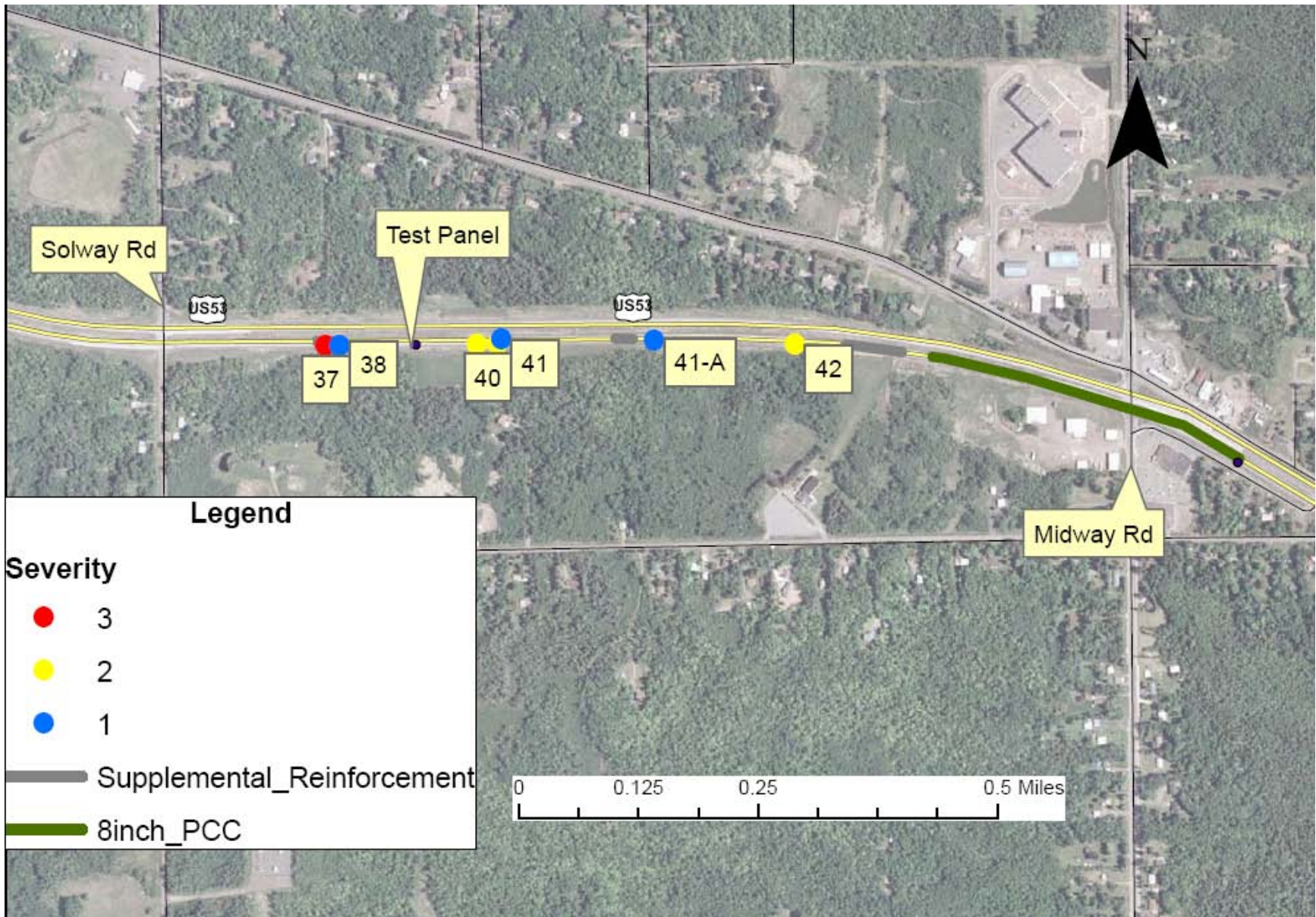
Figure 5.3. TH 53 Distress Map [Midway Rd to Solway Rd], April 2009 (Farm Service Agency, 2002)
