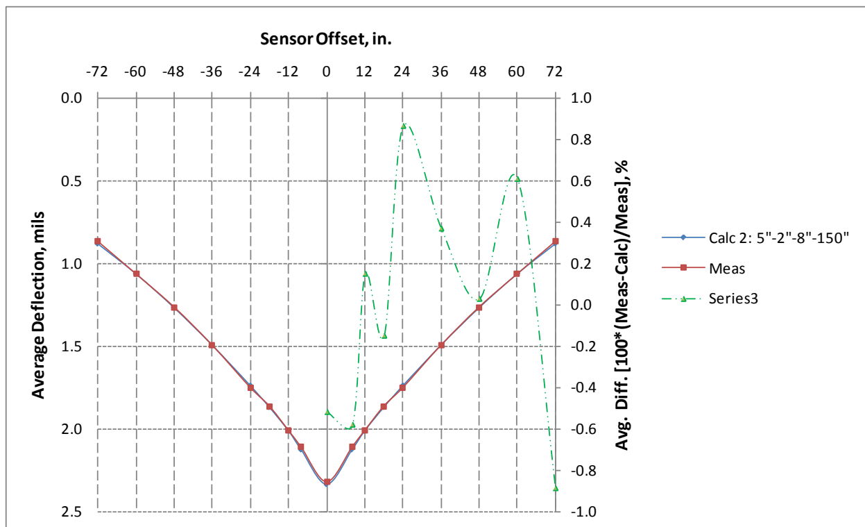
Figure 4.3. Comparison of EverCalc Calculated Deflections and the Measured Deflection
