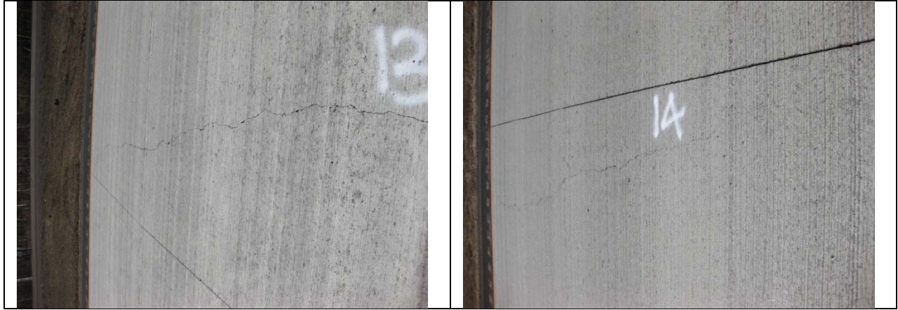
Figure A.7. Distress No. 13 [Left] & No. 14 [Right], April 2009
