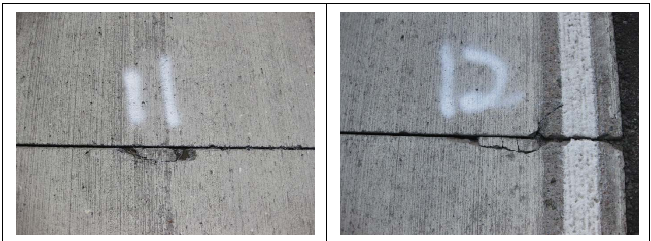
Figure A.6. Distress No. 11 [Left] & No. 12 [Right], April 2009
