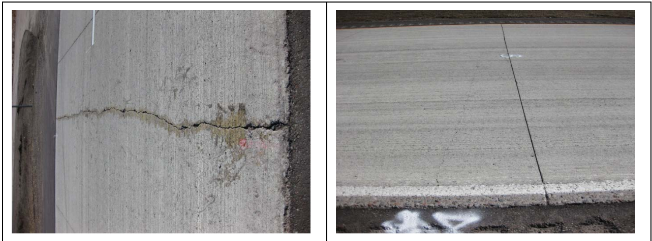
Figure A.2. Distress No. 3 [Left] & No. 4 [Right], April 2009
