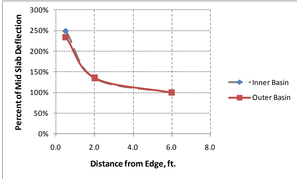
Figure 4.6. Comparison of the Deflections by Distance from Center of Slab
