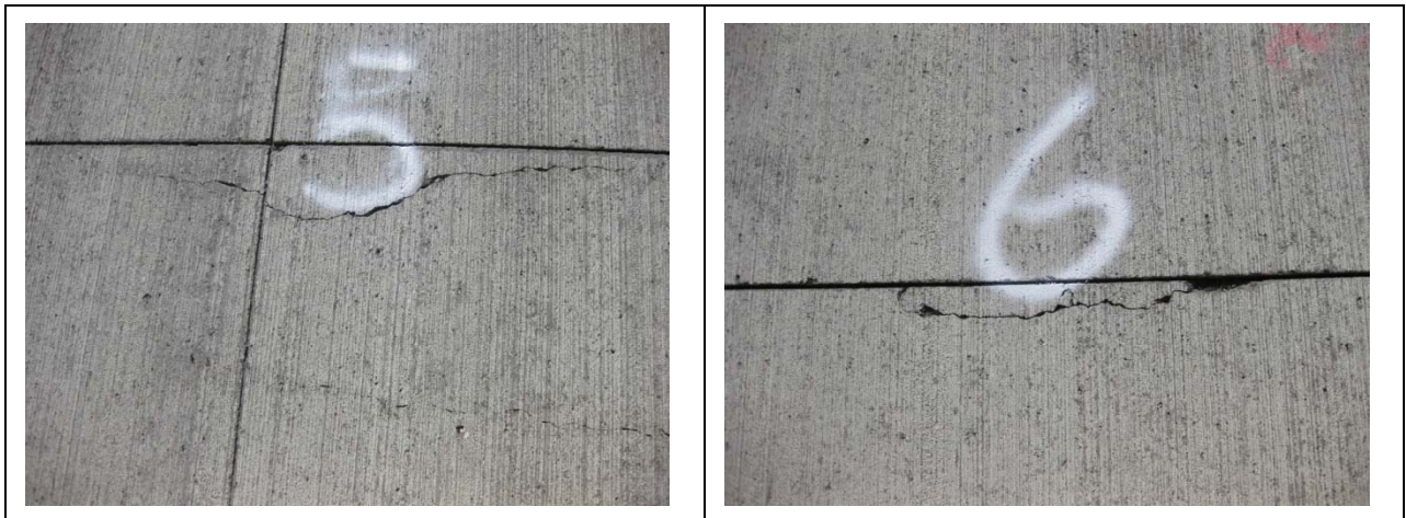
Figure A.3. Distress No. 5 [Left] & No. 6 [Right], April 2009
