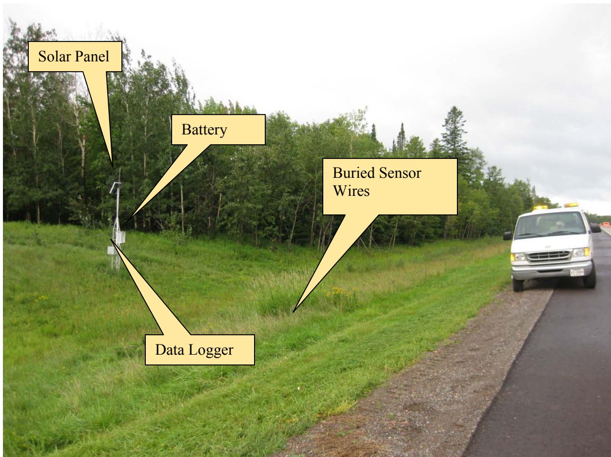
Figure 2.5. Completed Data Collection System
