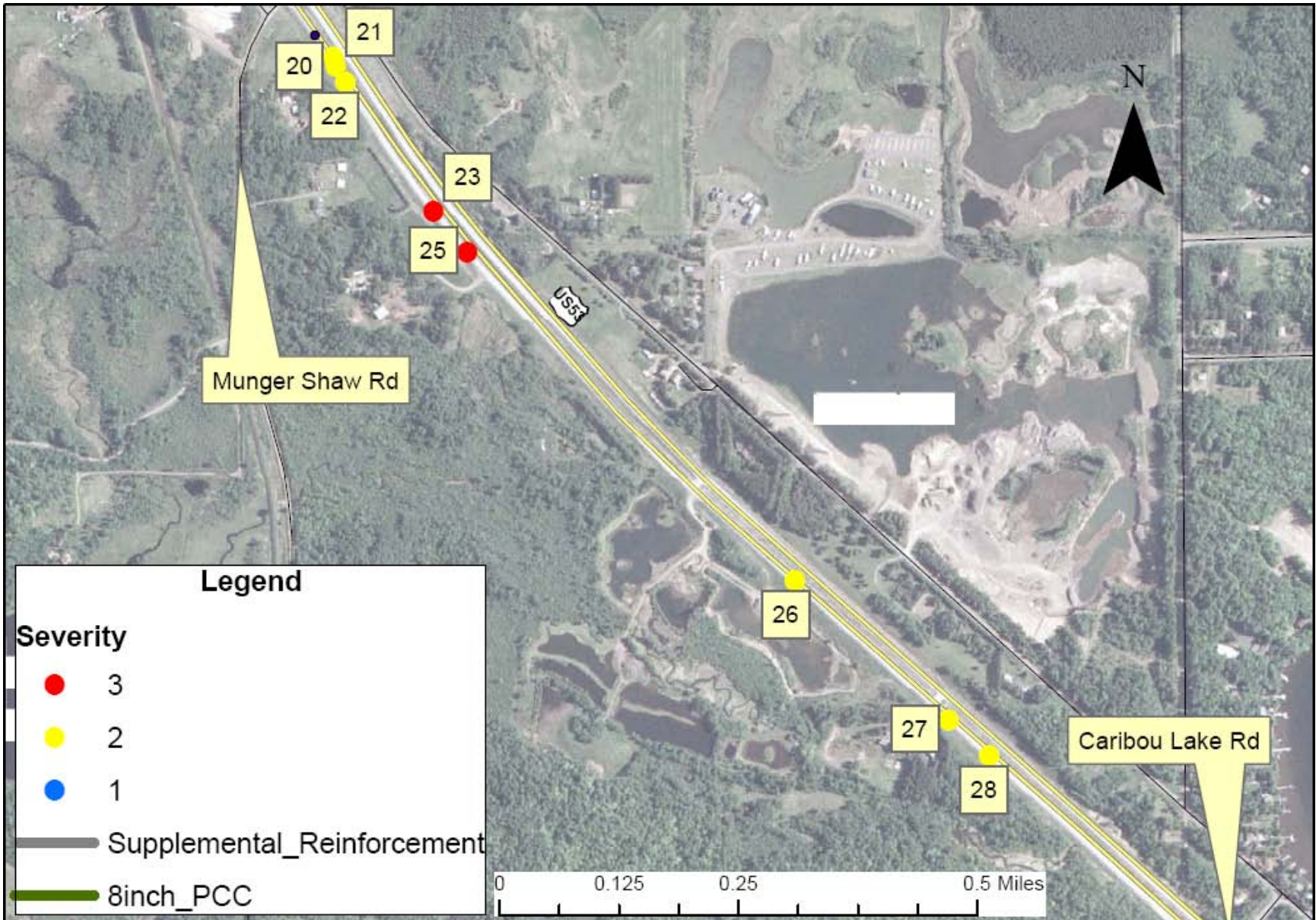
Figure 5.5. TH 53 Distress Map [Caribou Lake Rd to Munger Shaw Rd], April 2009 (Farm Service Agency, 2002)
