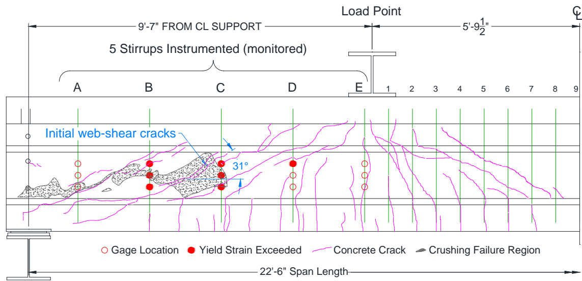
Figure A.11: Single girder 22.5 ft span west shear span cracking and failure
