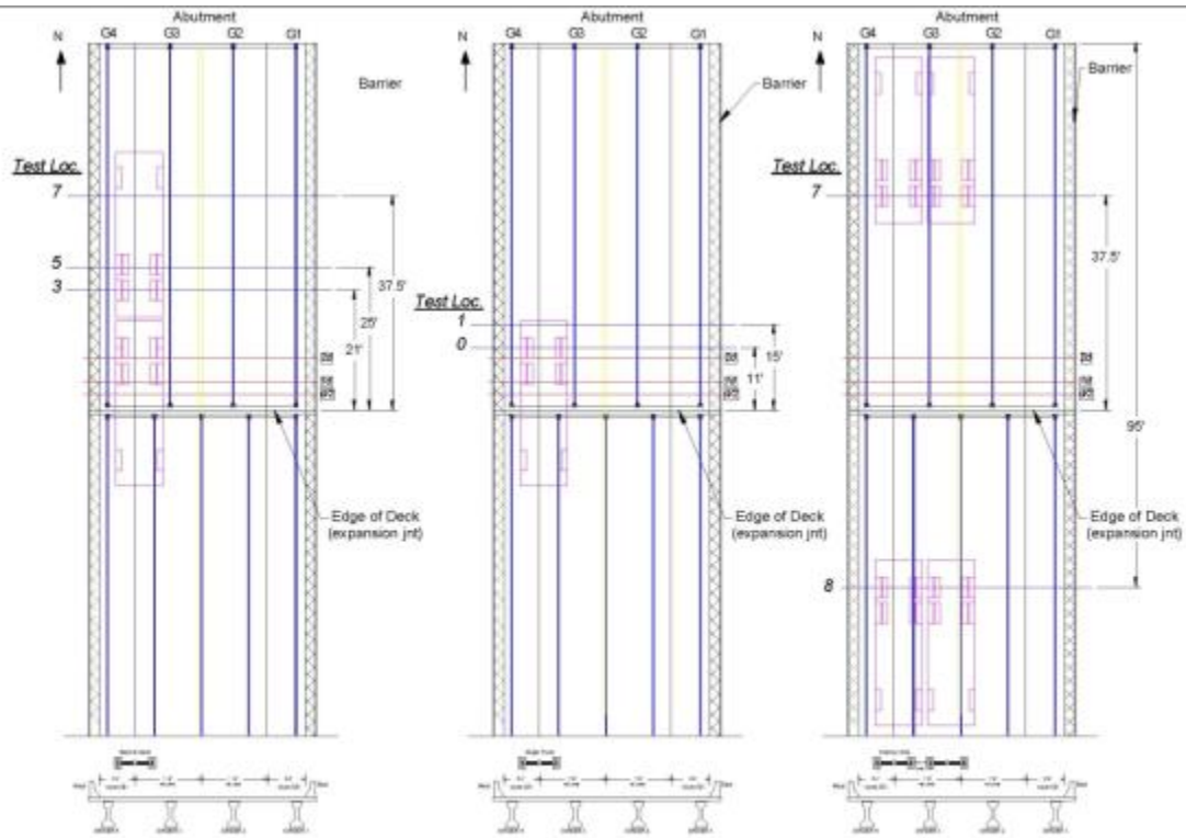
Figure 7. Exterior-Interior (G4-G3) Split Testing Locations
