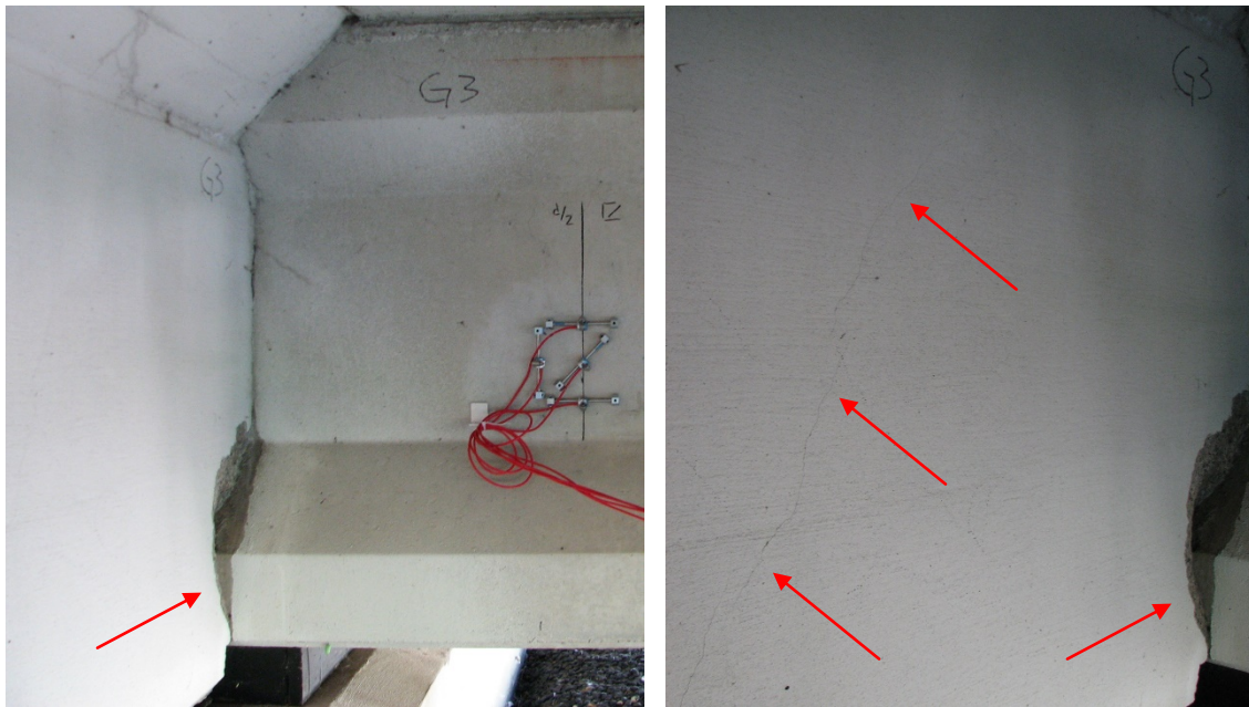
Figure 5.12: End diaphragm cracking observed in field bridge 73872
