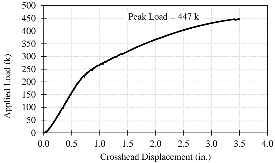
Figure F.17: Load-deflection plot for End B of the Bridge 62834 girder
