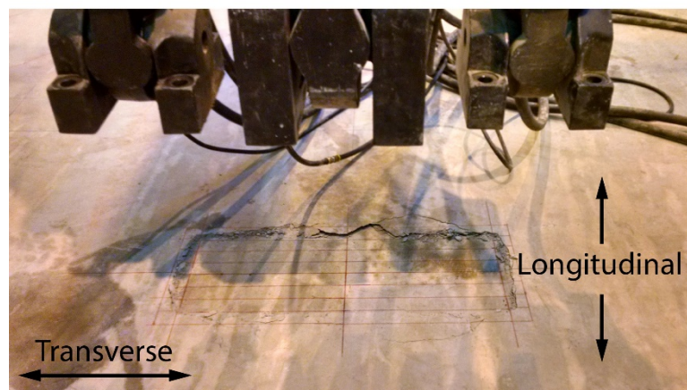
Figure 5.16: Typical deck punching surface above slab
