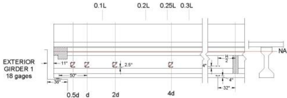
Figure 15. Girder 1 Instrumentation
