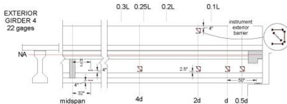
Figure 12. Girder 4 Instrumentation
