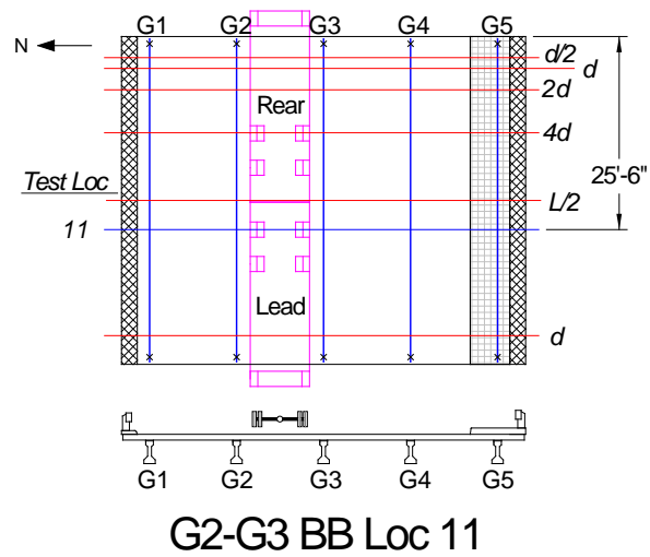
Figure 6.13: Loading cases for straight Bridge 09002 FEM validation
