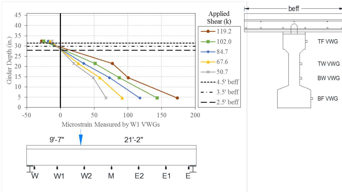
Figure A.26: Neutral axis height at W1 location for 30.75 ft span ( a/d = 2.5 )
