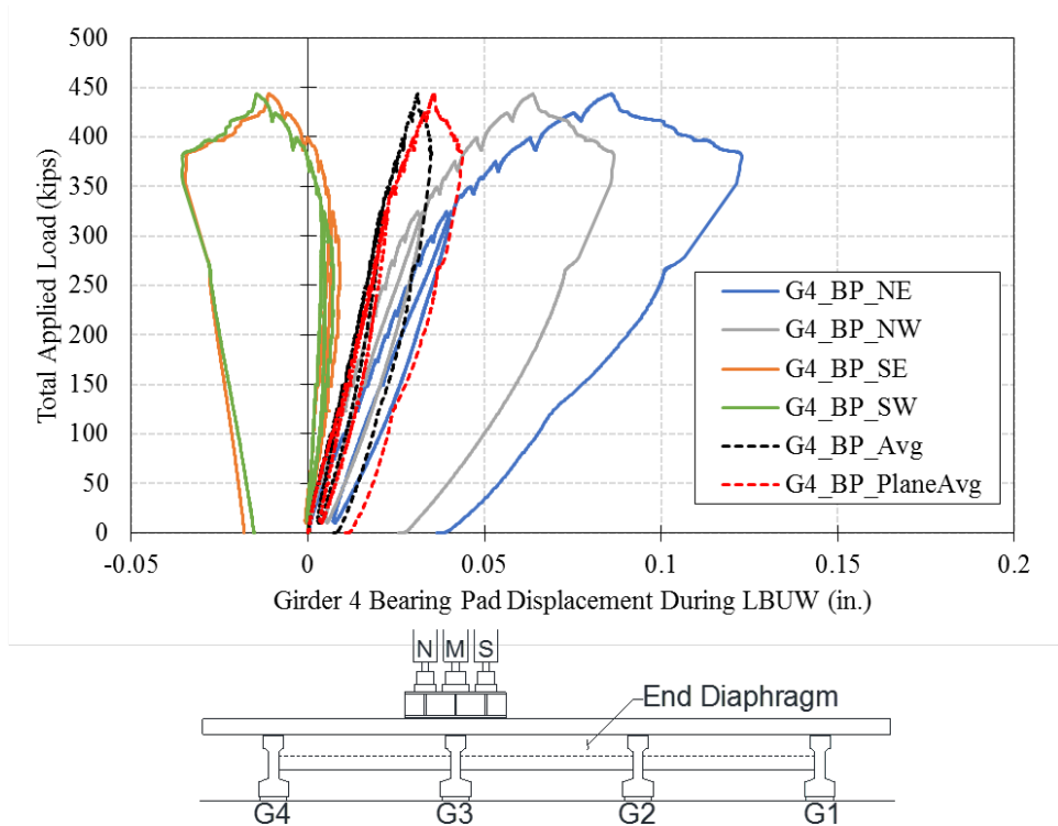
Figure E.4: Girder 4 bearing pad displacement during LBUW
