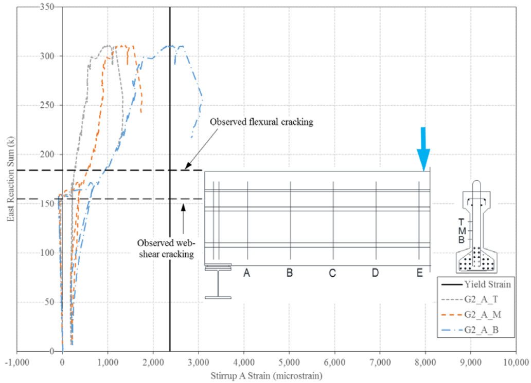
Figure E.24: Sum of east girder reactions vs. stirrup A strain for LBUE
