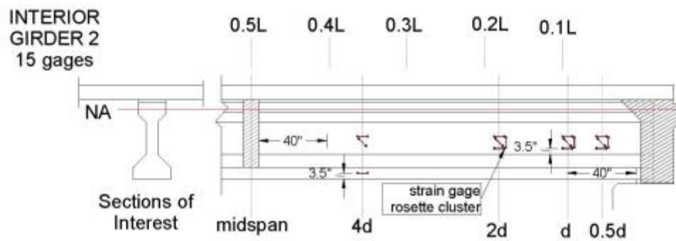
Figure 9. Girder 2 Instrumentation
