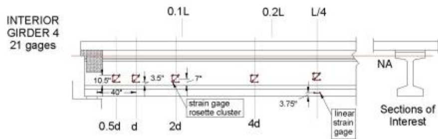
Figure 10. Girder 4 Instrumentation
