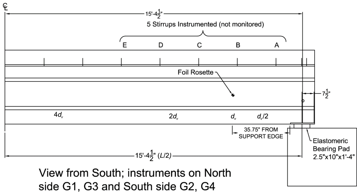
Figure 4.29: Instrumentation on east half of span for LBUW
