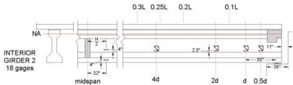
Figure 14. Girder 2 Instrumentation
