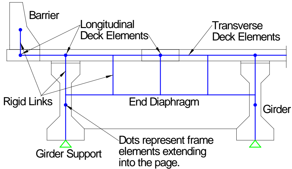
Figure 3.1: Cross section of three-dimensional grillage frame elements
