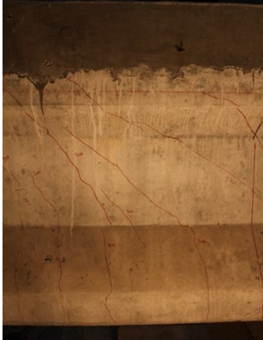
Figure F.15: Photograph of Bridge 62384 girder (End A) at end of test showing first observed shear cracks, which occurred near applied load in long shear span
