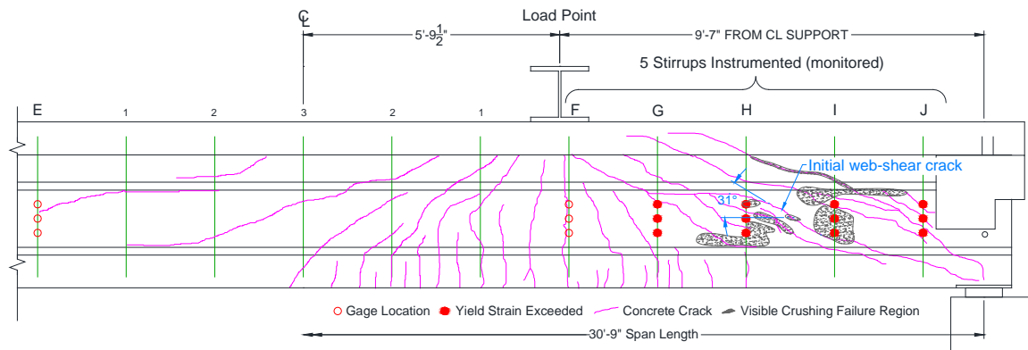
Figure 5.13: Girder 3 northwest cracking and failure from LBUW looking south
