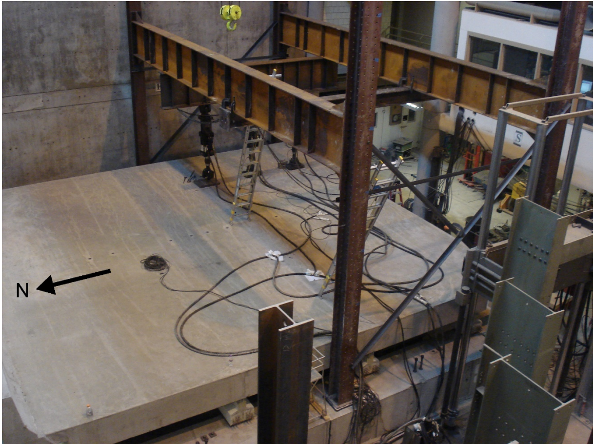
Figure 4.32: Steel load frame configured for LBESE testing
