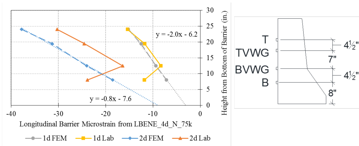
Figure 5.8: Barrier longitudinal strain through section at 1d_v and 2d_v for LBENE
