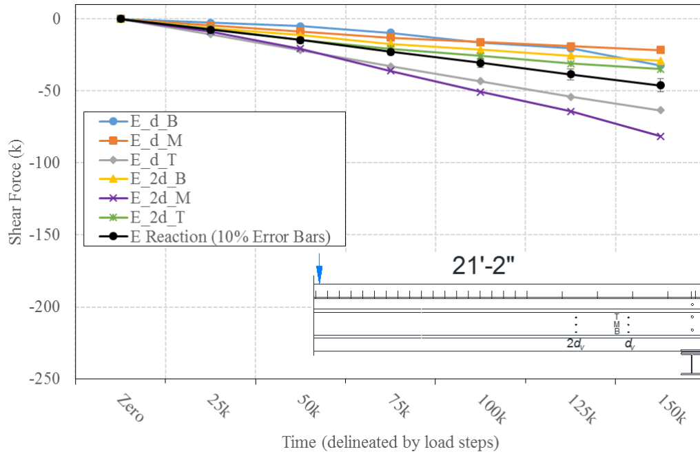
Figure A.19: Elastic force derived from foil rosette strains in 21 ft 2 in. shear span for 30.75 ft span
