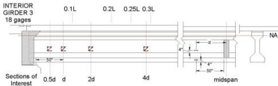
Figure 13. Girder 3 Instrumentation
