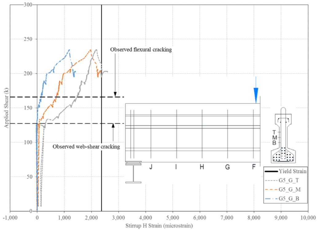
Figure A.22: Applied shear vs. stirrup G strain for 30.75 ft span ( a/d = 2.5 )
