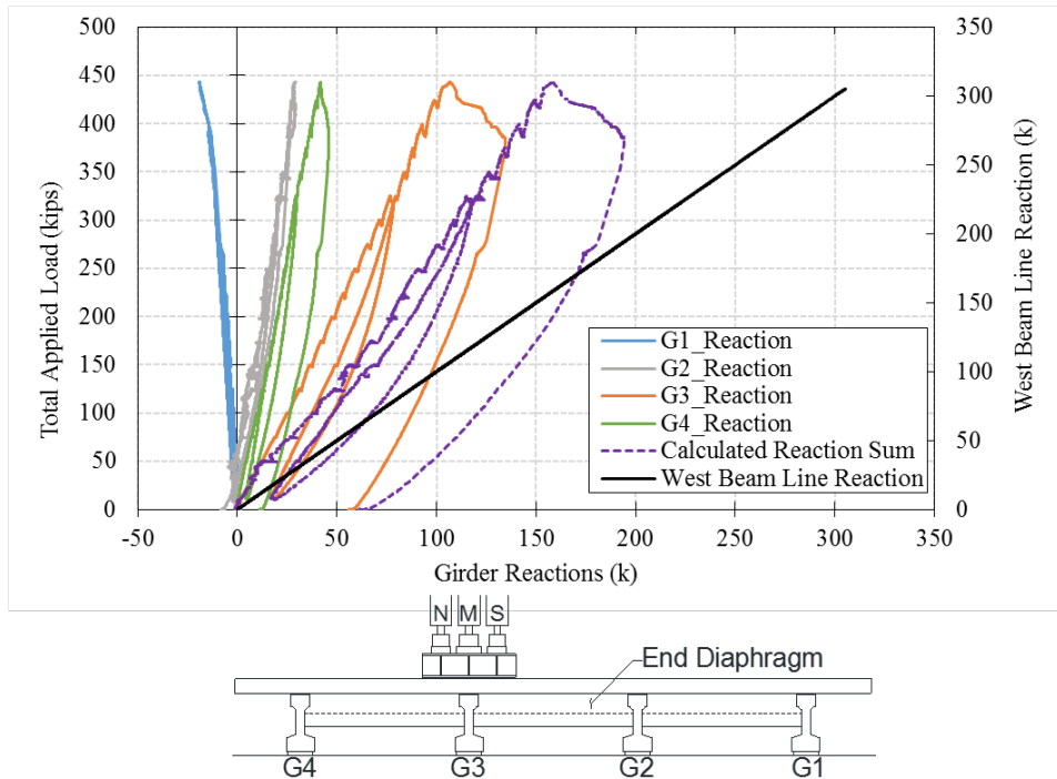
Figure E.7: Girder reactions estimated with bearing pad LVDT data for LBUW
