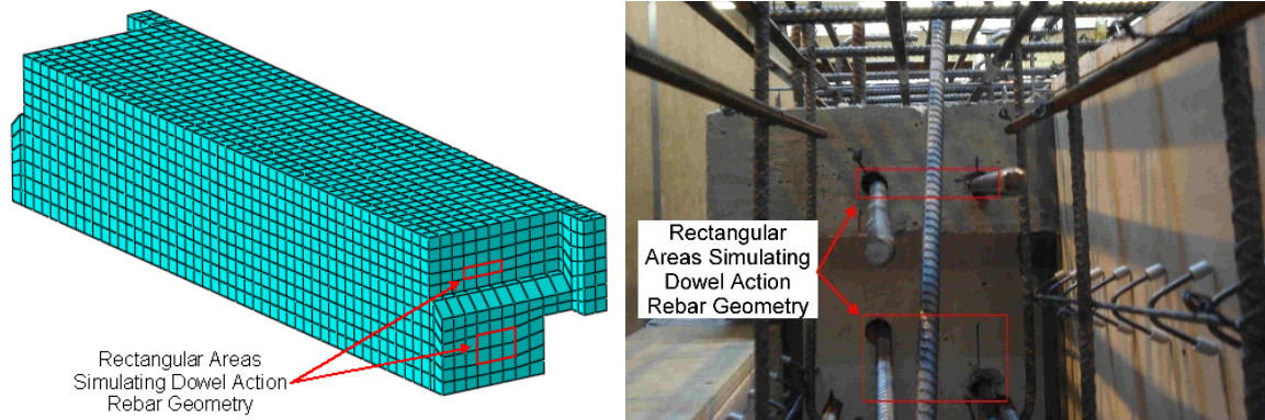
Figure 5.5: End diaphragm pinned fixity simulating as-built connectivity
