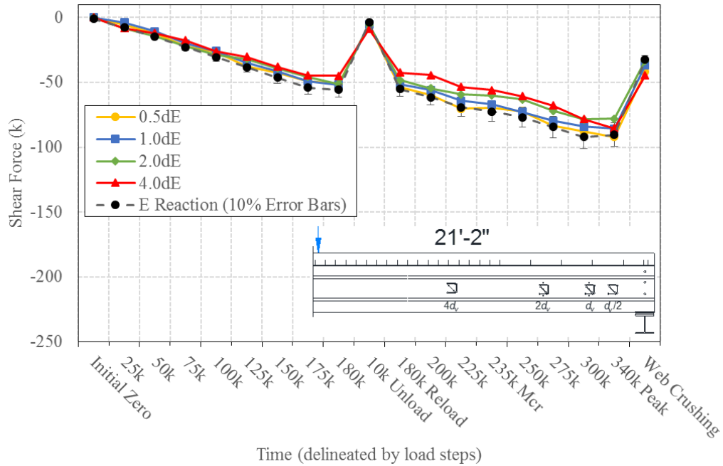
Figure A.17: Elastic force derived from VWG rosette strains in 21 ft 2 in. shear span for 30.75 ft span
