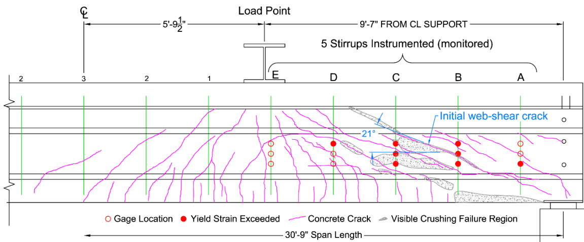
Figure 5.19: Girder 2 southeast cracking and failure from LBUW looking north
