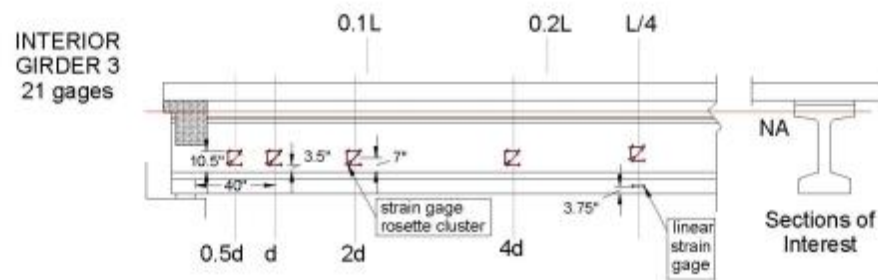
Figure 11. Girder 3 Instrumentation
