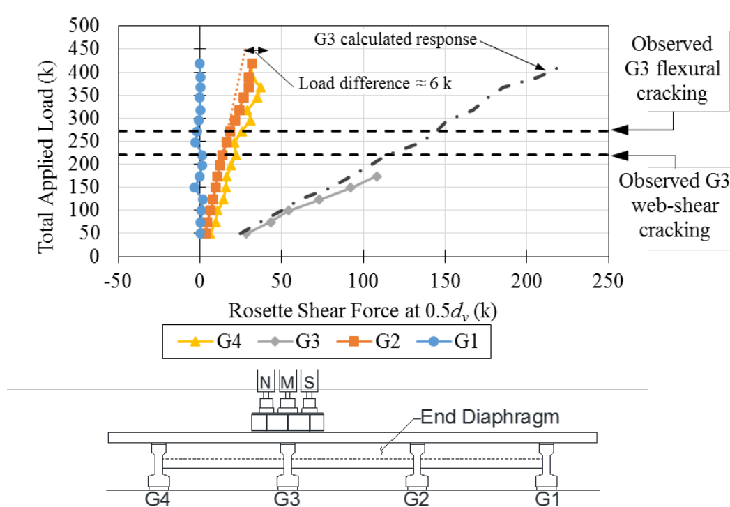
Figure 5.21: Shear redistribution at 0.5d_v during LBUE
