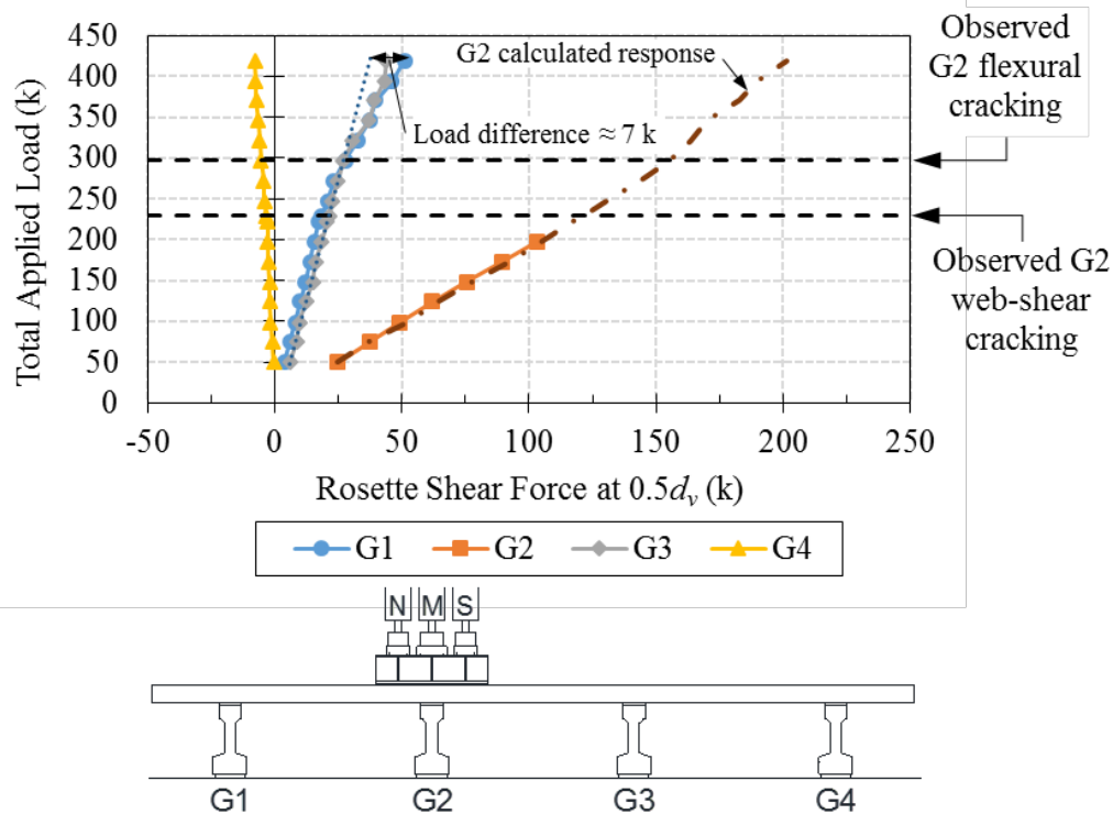
Figure 5.24: Shear redistribution at 0.5d_v during LBUE
