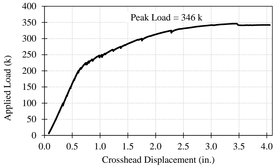
Figure F.7: Load-deflection plot for the Bridge 27799L girder
