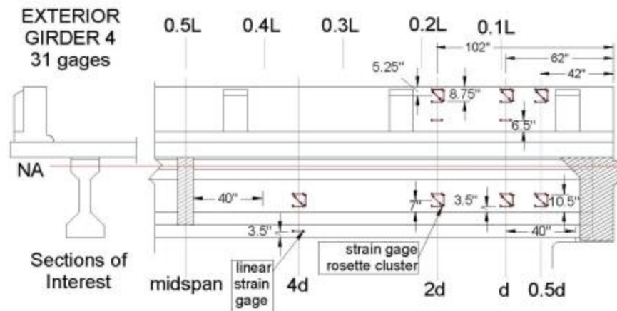
Figure 7. Girder 4 Instrumentation
