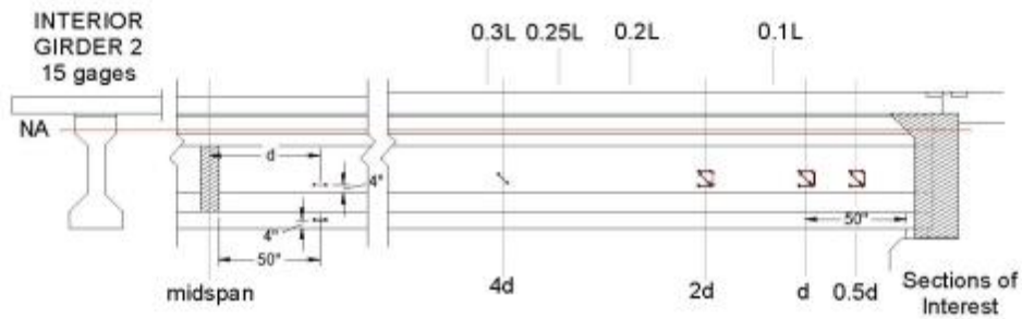
Figure 14. Girder 2 Instrumentation
