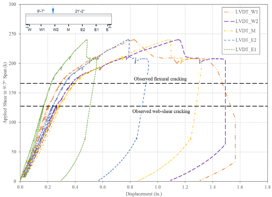
Figure A.34: Applied shear vs. displacement for 30.75 ft span ( a/d = 2.5 )
