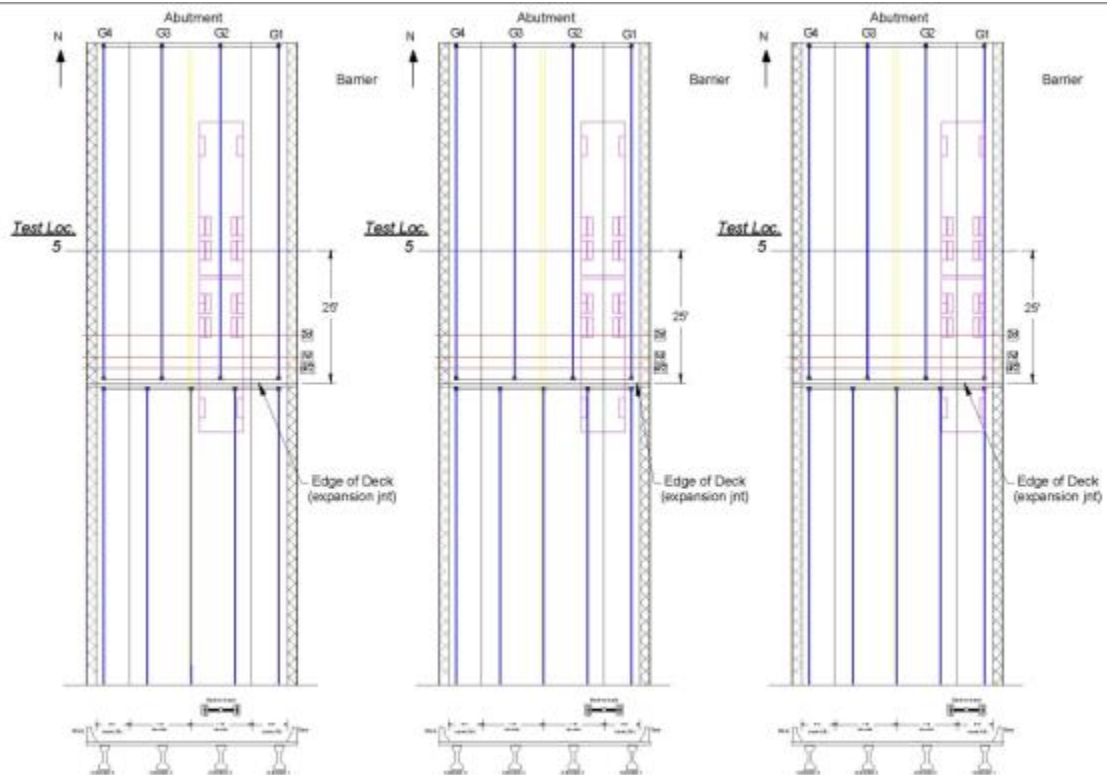
Figure 9. Symmetric Girder (G2, G2-G1 split, and G1) Testing Locations
