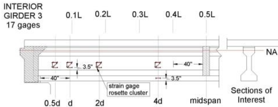
Figure 8. Girder 3 Instrumentation
