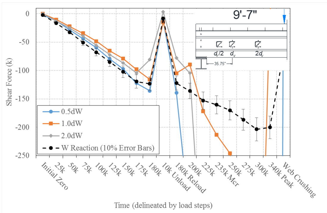
Figure A.16: Elastic force derived from VWG rosette strains in 9 ft 7 in. shear span for 30.75 ft span
