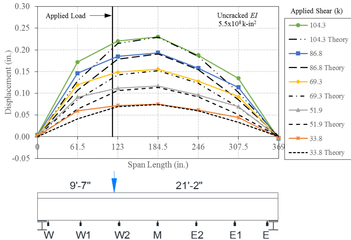
Figure A.35: Elastic displacement profile with varying load for 30.75 ft span ( a/d = 2.5 )
