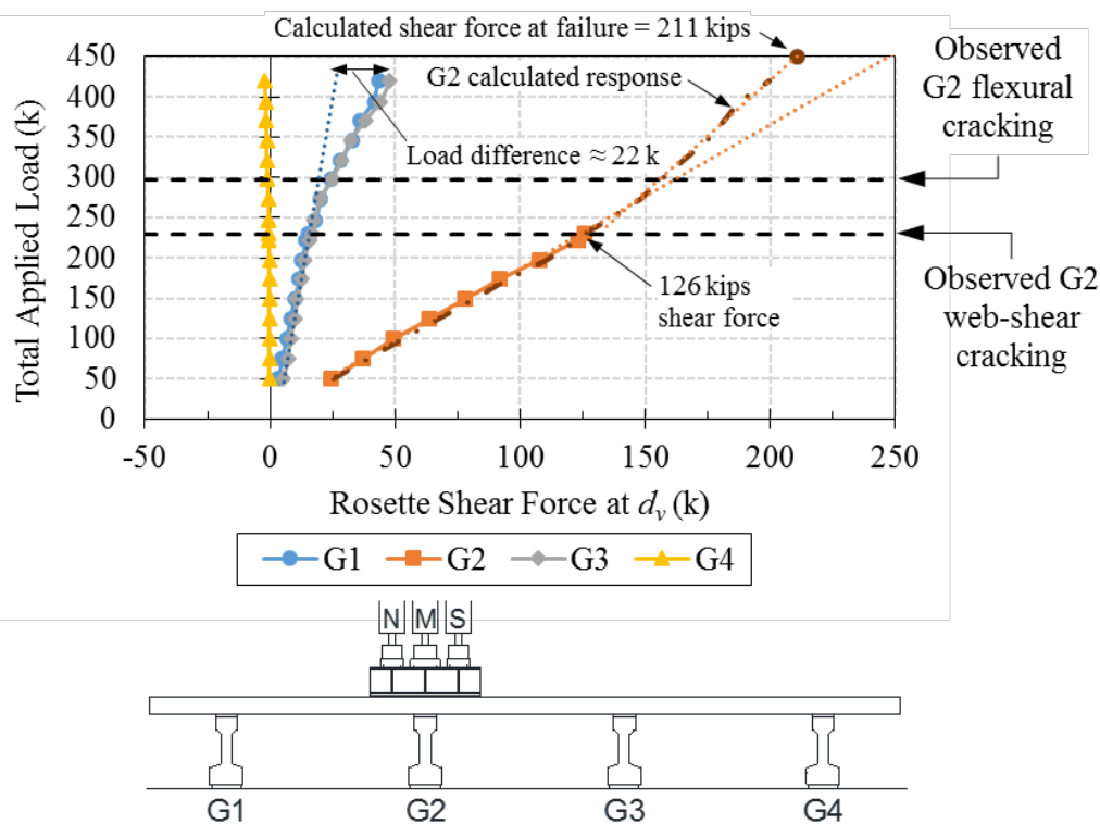
Figure 5.25: Shear redistribution at d_v during LBUE
