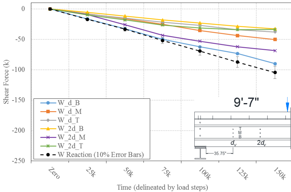
Figure A.18: Elastic force derived from foil rosette strains in 9 ft 7 in. shear span for 30.75 ft span
