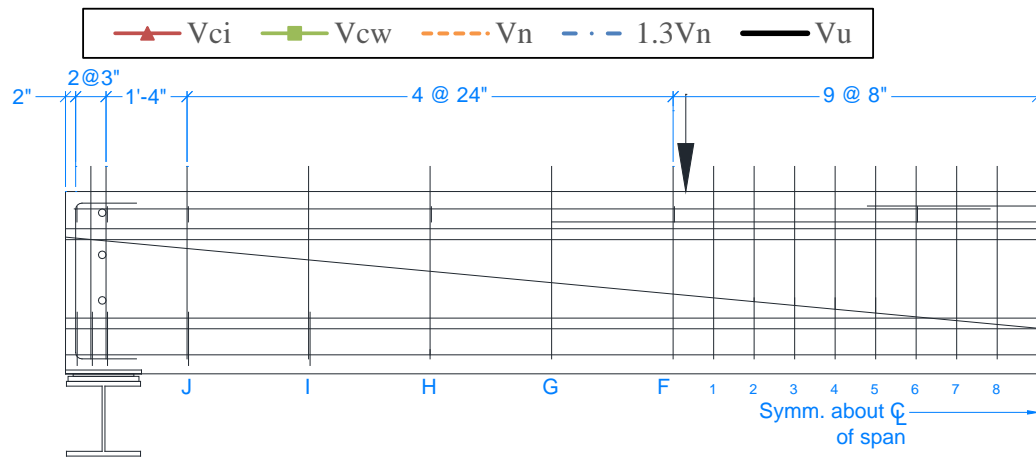
Figure A.12: Shear force diagram for 30.75 ft span
