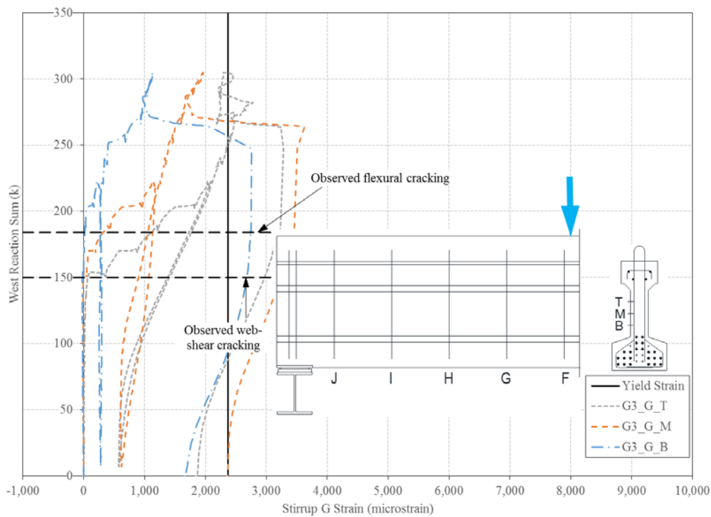
Figure E.23: Sum of west girder reactions vs. stirrup G strain for LBUW
