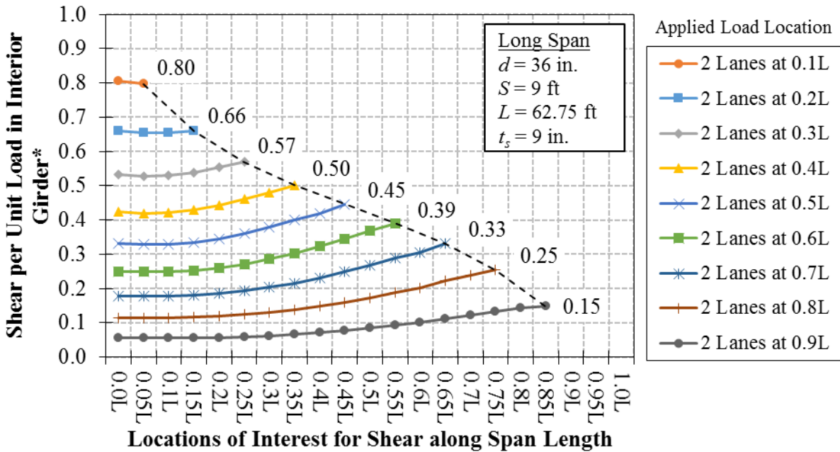
Figure I.12: Long span shear per unit load vs. span length for 2 lanes loaded
