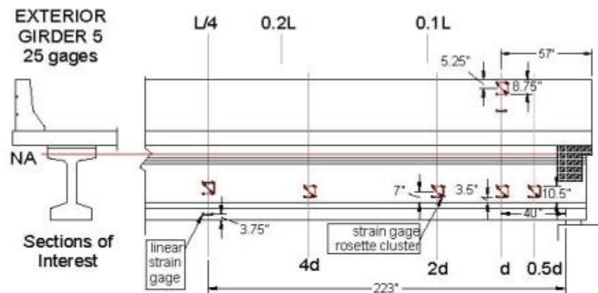
Figure 9. Girder 5 Instrumentation
