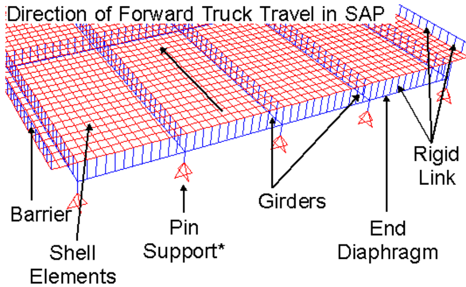
Figure 3.3: Three-dimensional grillage model with shell elements for bridge deck
