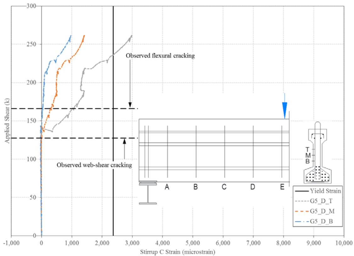
Figure A.25: Applied shear vs. stirrup D strain for 22.5 ft span ( a/d = 2.5 )
