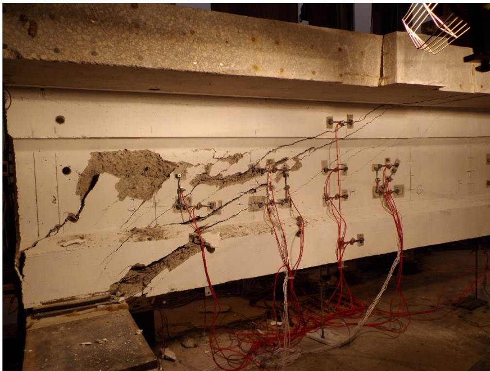
Figure A.14: Web-shear crushing failure in 30.75 ft span
