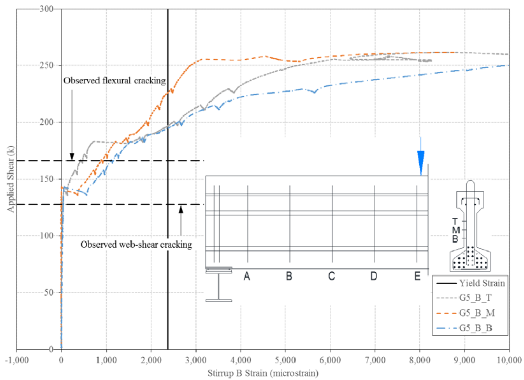
Figure A.23: Applied shear vs. stirrup B strain for 22.5 ft span ( a/d = 2.5 )
