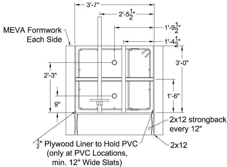
Figure B.4: Cross section of abutment formwork and non-reinforcement details
