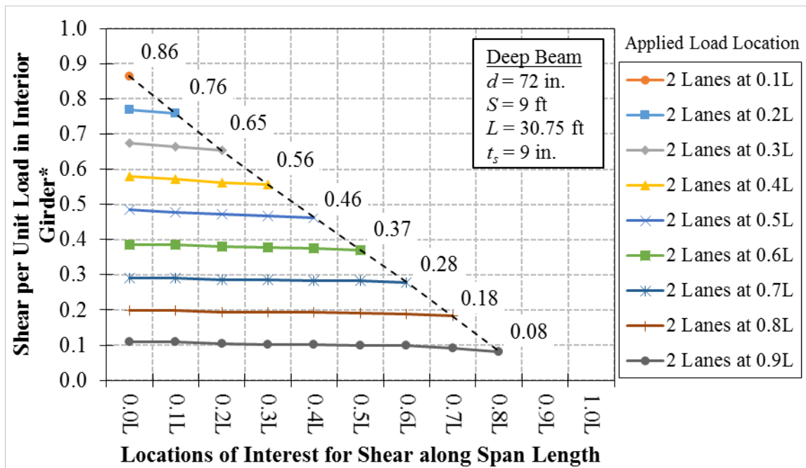
Figure I.9: Deep beam shear per unit load vs. span length for 2 lanes loaded
