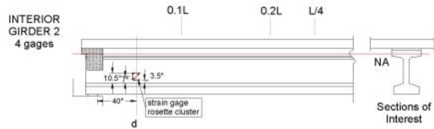
Figure 12. Girder 2 Instrumentation
