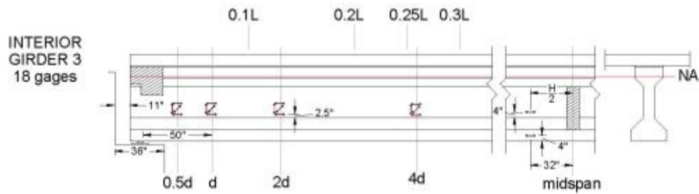
Figure 13. Girder 3 Instrumentation
