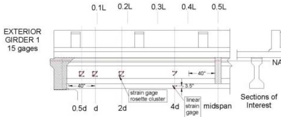
Figure 10. Girder 1 Instrumentation
