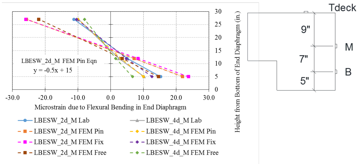
Figure 5.11: Comparison of end diaphragm neutral axis for LBESW
