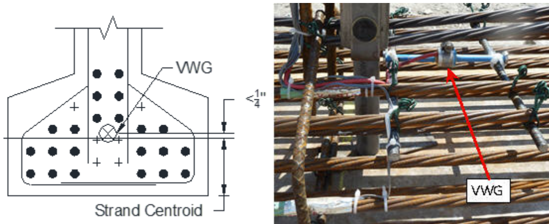
Figure 4.17: Location of internal vibrating wire strain gages
