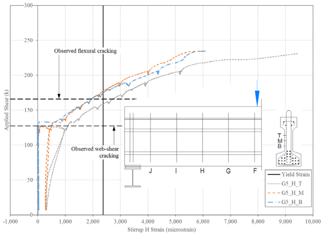
Figure A.21: Applied shear vs. stirrup H strain for 30.75 ft span ( a/d = 2.5 )
