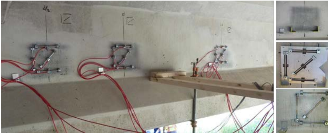
Figure 4.26: Example box-type rosette VWGs
