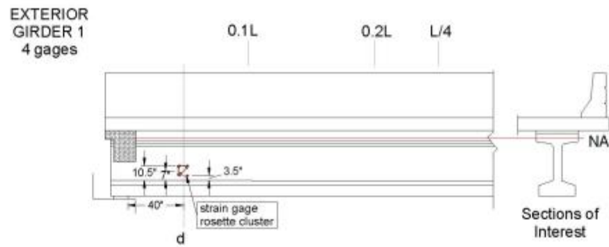
Figure 13. Girder 1 Instrumentation
