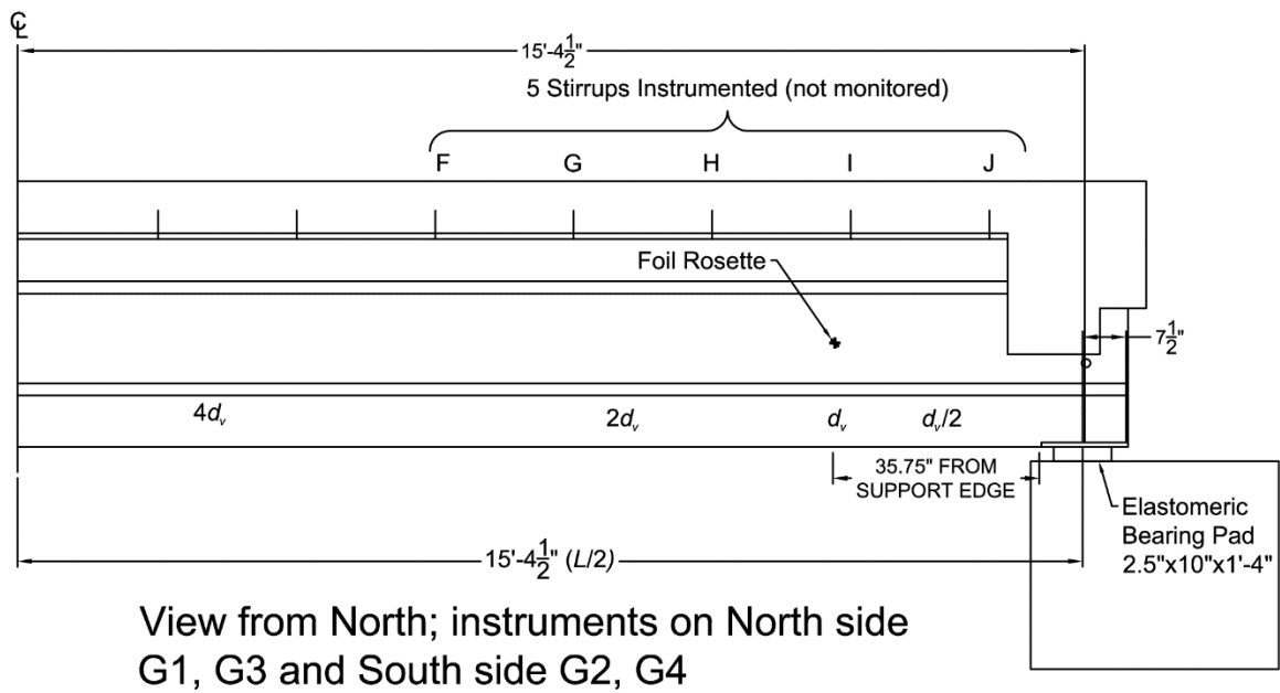
Figure 4.31: Instrumentation on west half of span for LBUE
