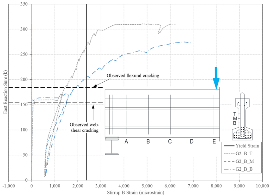
Figure E.25: Sum of east girder reactions vs. stirrup B strain for LBUE
