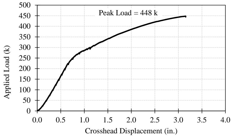
Figure F.13: Load-deflection plot for End A of the Bridge 62834 girder
