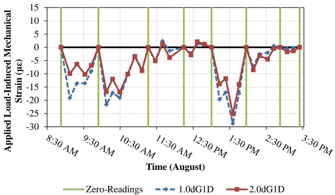
Figure 6.9: Applied load-induced mechanical strain only from Bridge 09002
