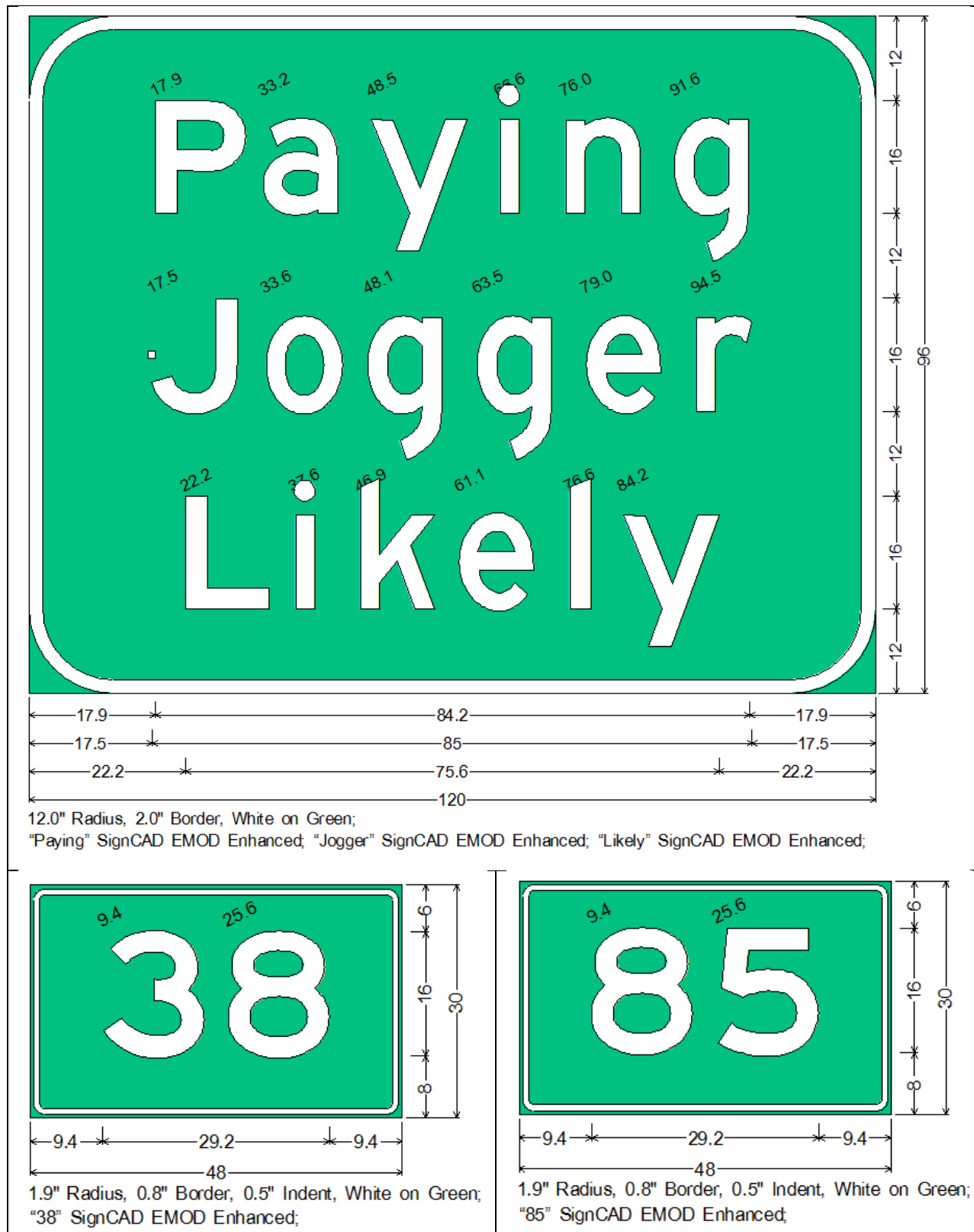
Figure B.3. Enhanced E(Mod) Sign Layouts.
