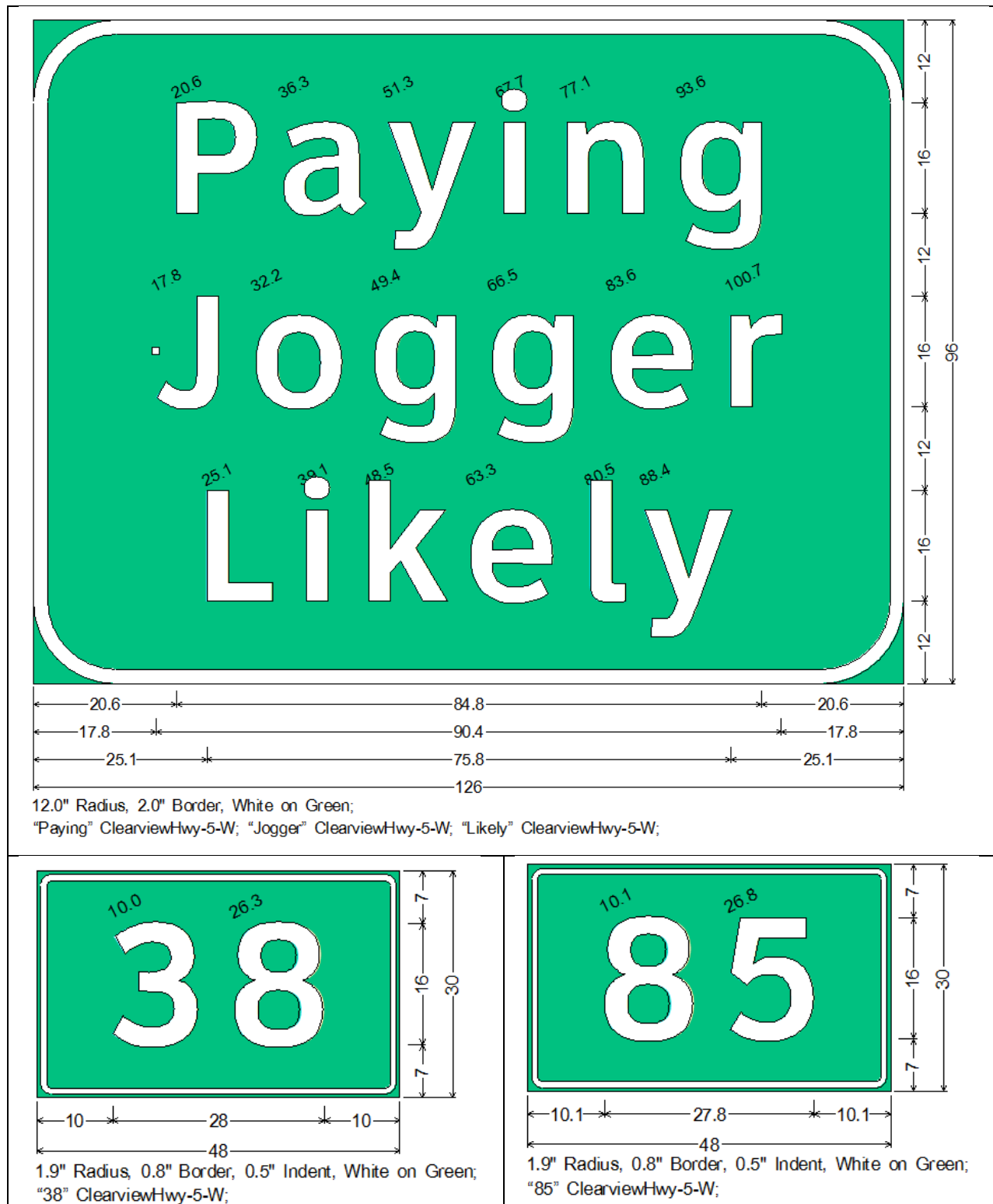
Figure B.2. Clearview 5W Sign Layouts.
