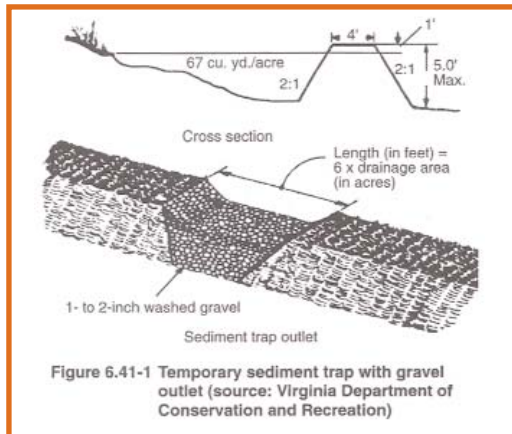
Figure 6.41-1 Temporary sediment trap with gravel outlet (source: Virginia Department of Conservation and Recreation) Temporary sediment traps are useful as velocity checks and treatment areas. Source: Minnesota Pollution Control Agency Best Management Practices Manual, 2000
