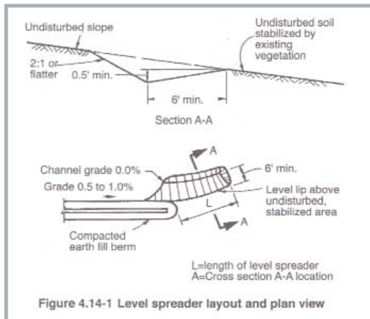
Typical runoff spreader design. Source: Minnesota Pollution Control Agency Best Management Practices Manual 2000
